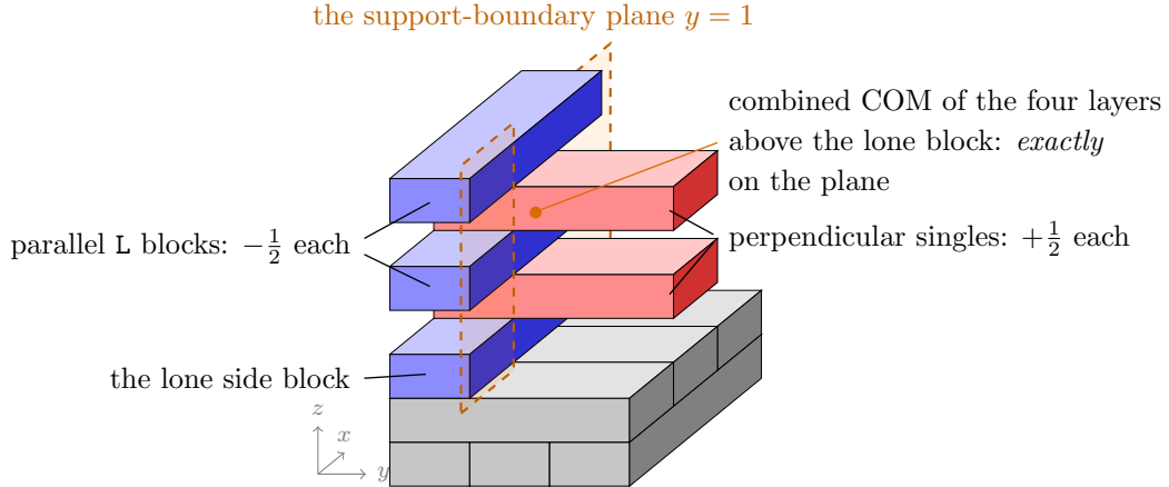
Figure 2: The knife-edge configuration. The lone side block's support ends at the plane y = 1 ; each perpendicular layer's unavoidable +\frac{1}{2} exactly cancels each parallel layer's best possible -\frac{1}{2} , parking the centre of mass of everything above precisely on the boundary.
