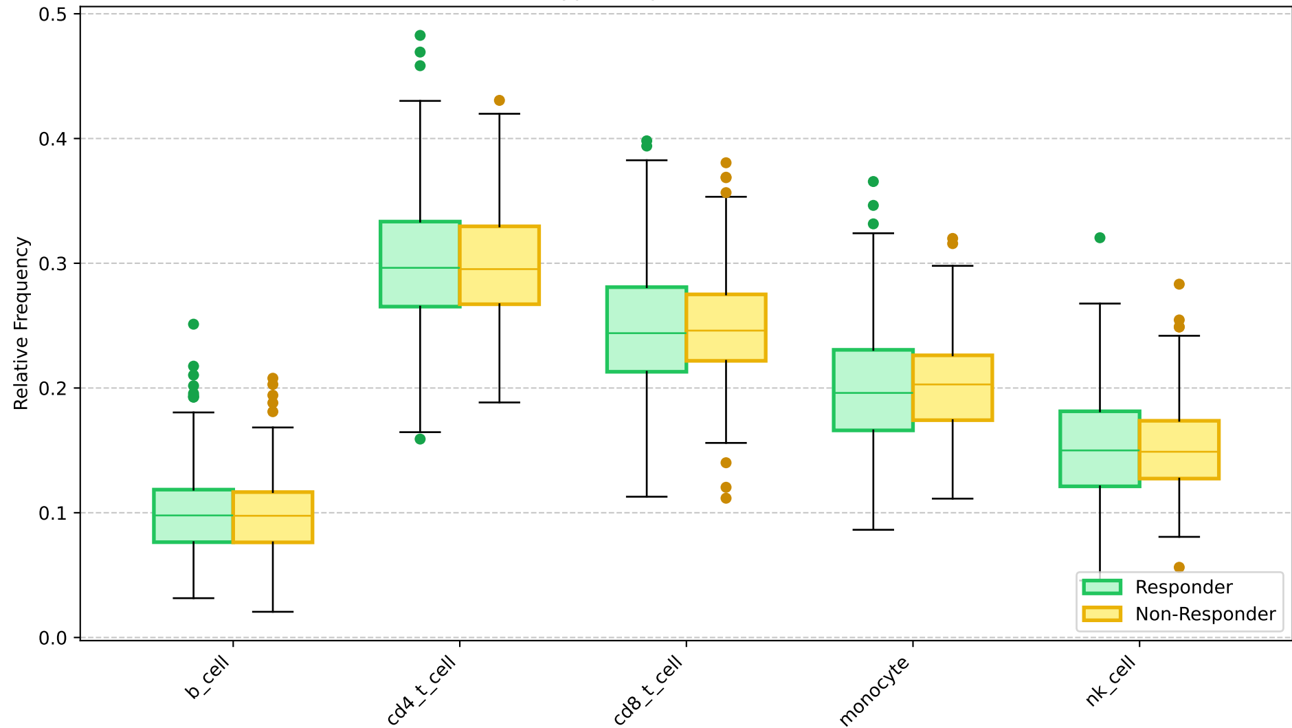
Cell Type Frequencies at Baseline
