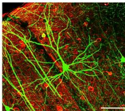
A Brain
