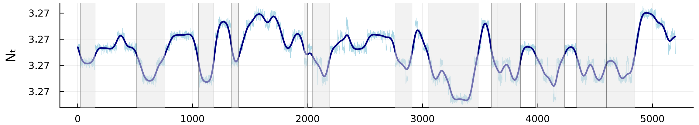
Job-filling rate
