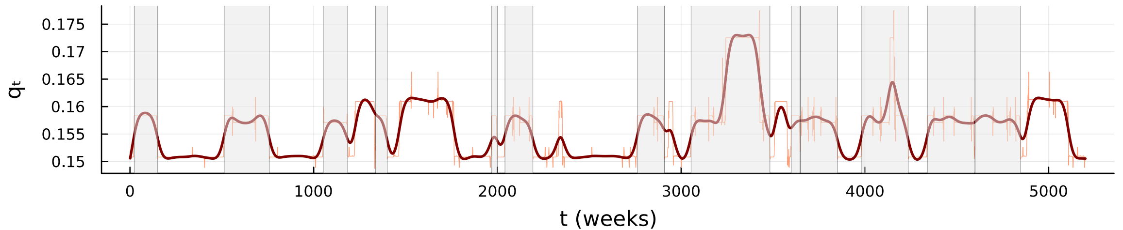
Job-filling rate
