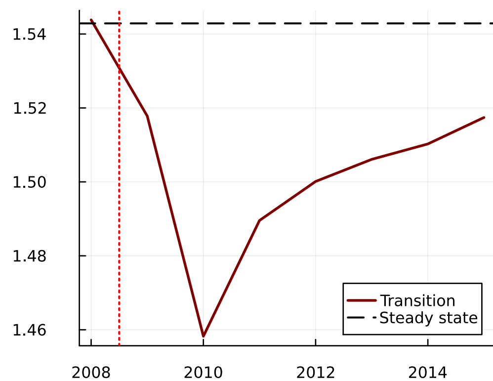
W_t
