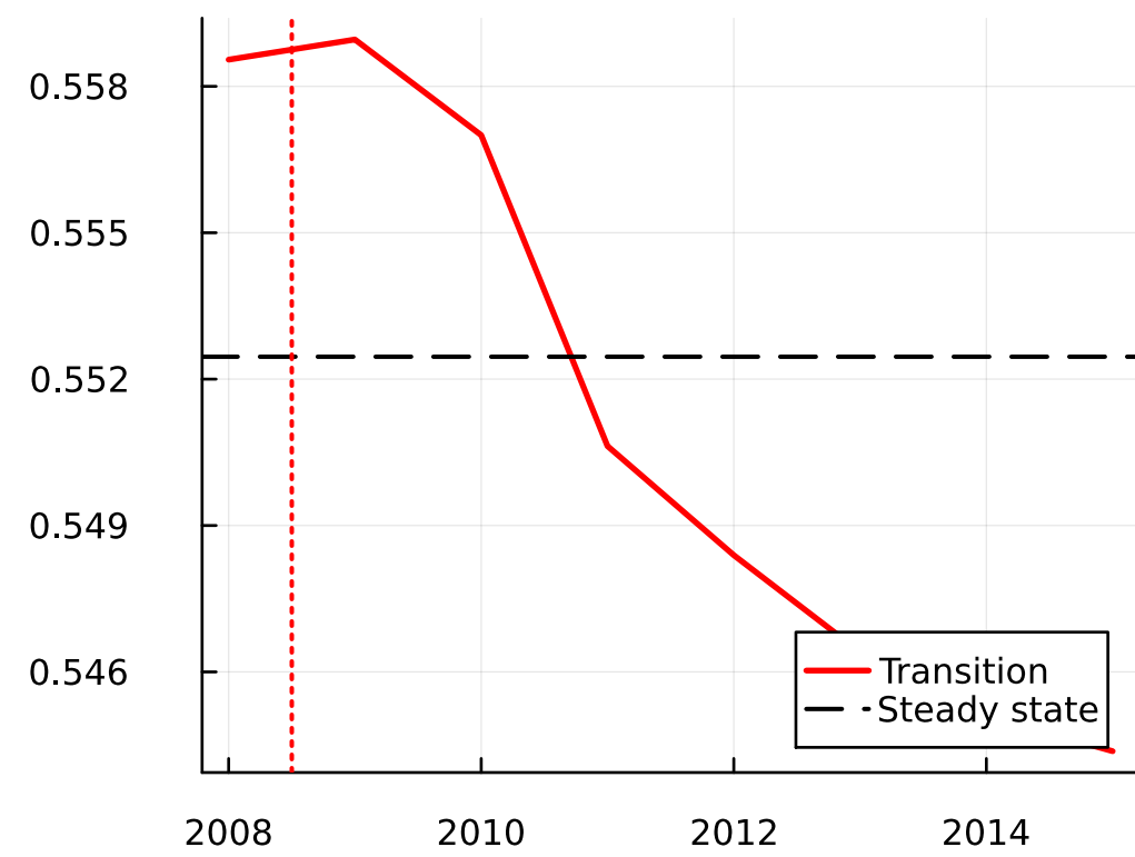
\tau
