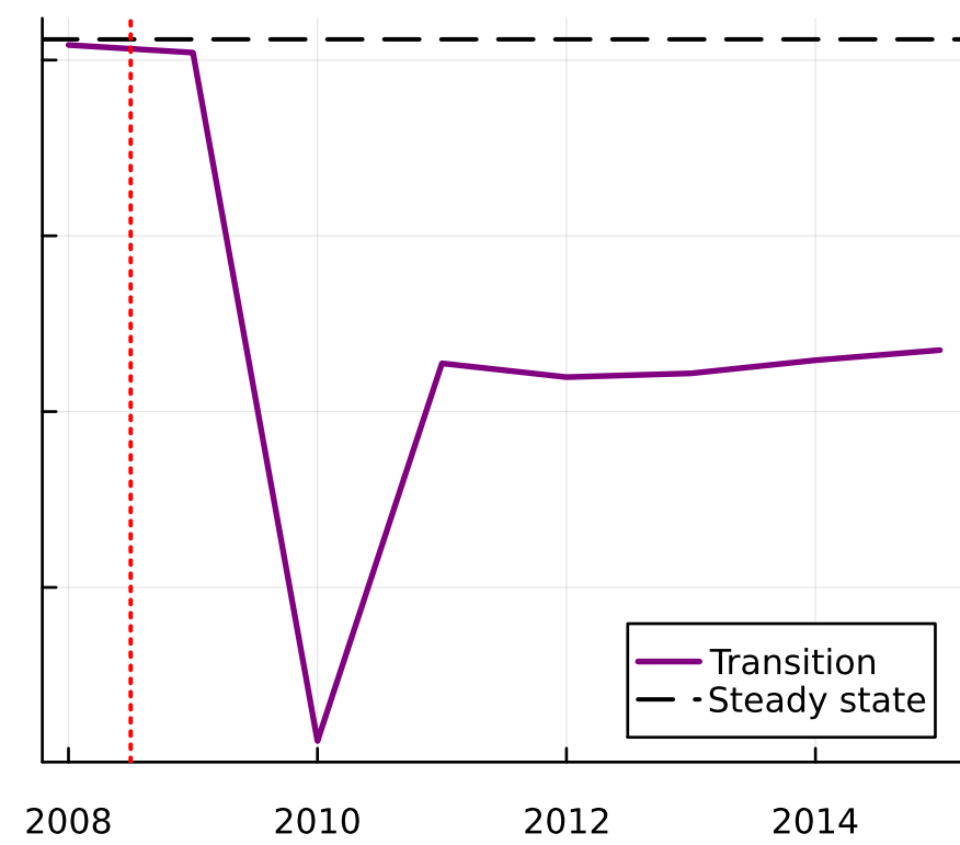
W_t
