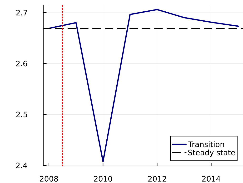
\mathbb{E}[z]
