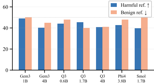
(b) Exp 1: HarmBench — Gemma 3 / Qwen 3 / Others
