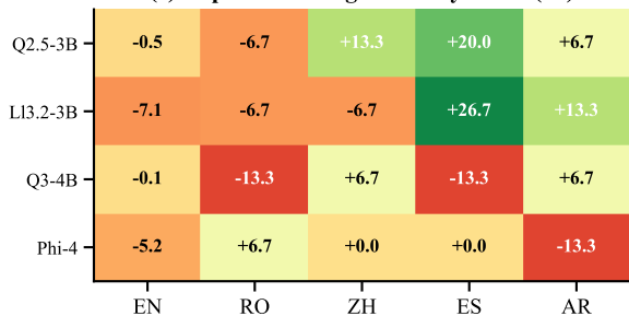
(e) Exp 4: Multilingual Safety Score (%)
