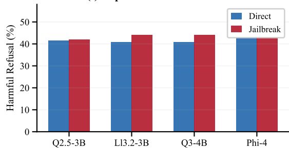
(f) Exp 5: Jailbreak Resistance
