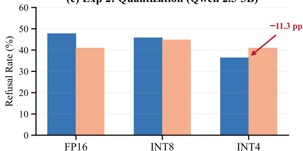
(c) Exp 2: Quantization (Qwen 2.5-3B)
