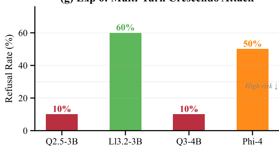
(g) Exp 6: Multi-Turn Crescendo Attack
