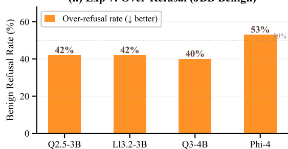
(h) Exp 7: Over-Refusal (JBB Benign)
