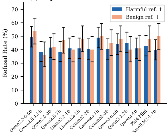
(a) Exp 1: HarmBench size-stratified
