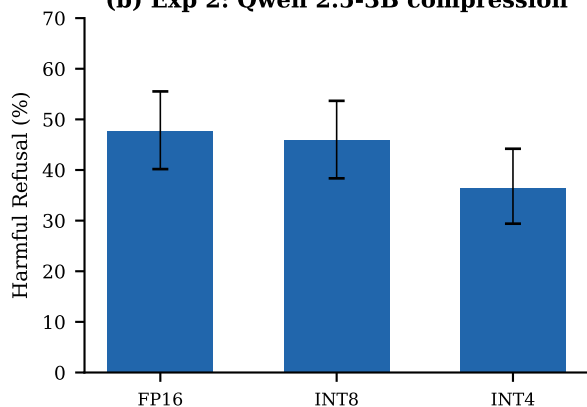
(b) Exp 2: Qwen 2.5-3B compression
