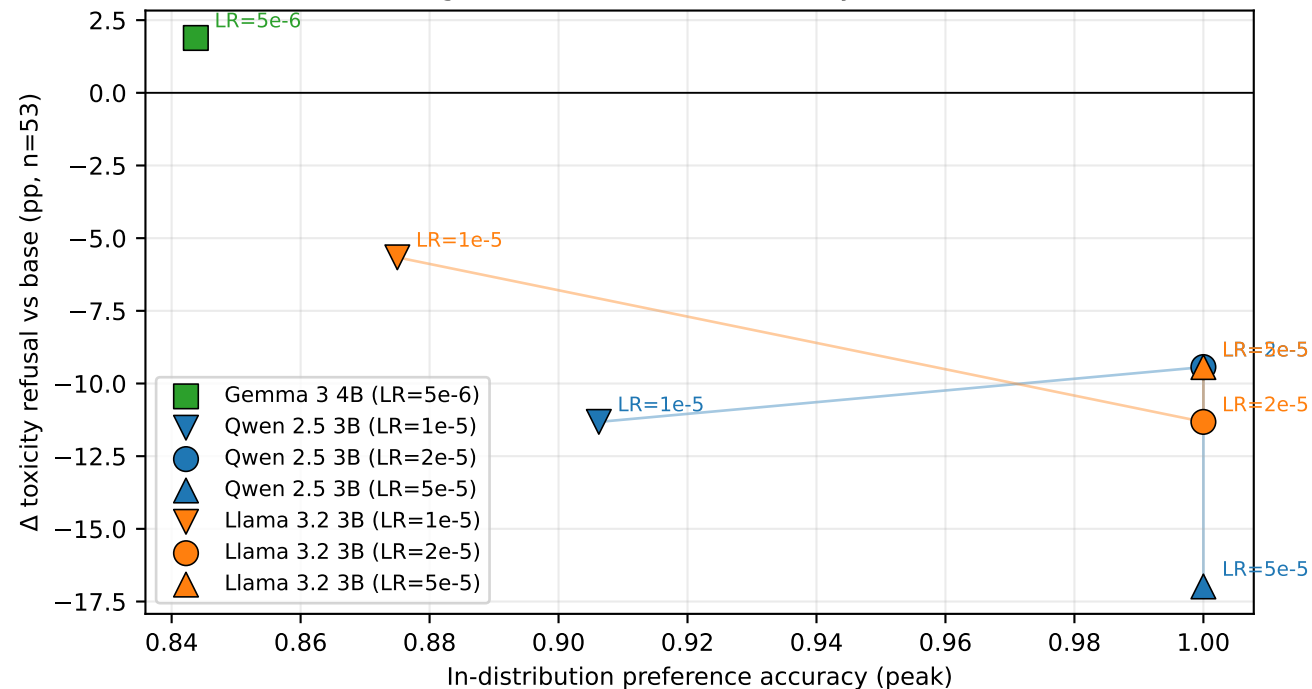
Training harder makes OOD toxicity refusal worse
