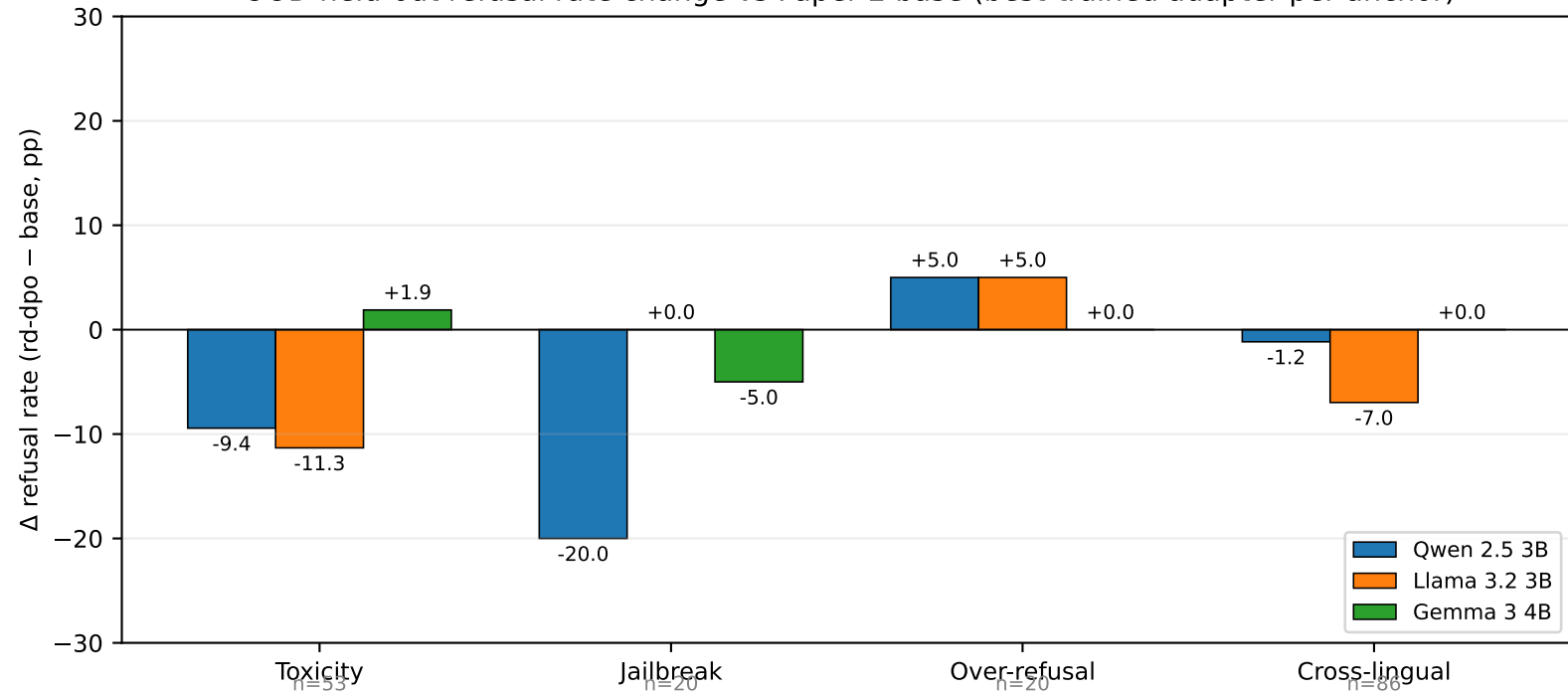
OOD held-out refusal rate change vs Paper 2 base (best-trained adapter per anchor)
