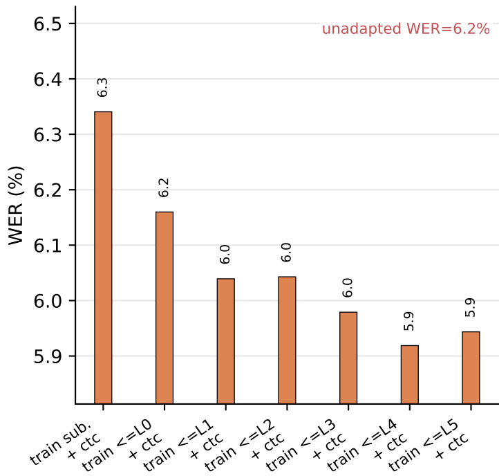
TED-LIUM
