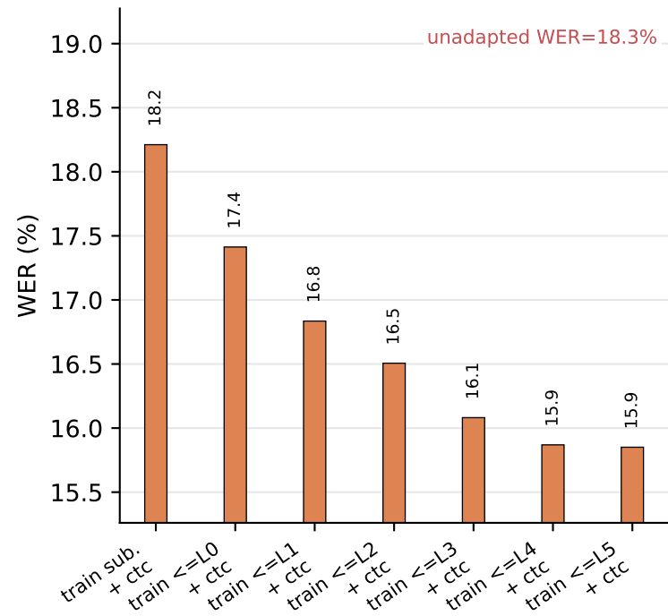
Earnings22
