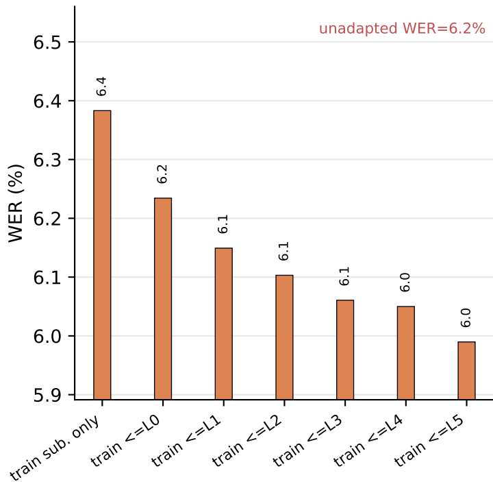
TED-LIUM
