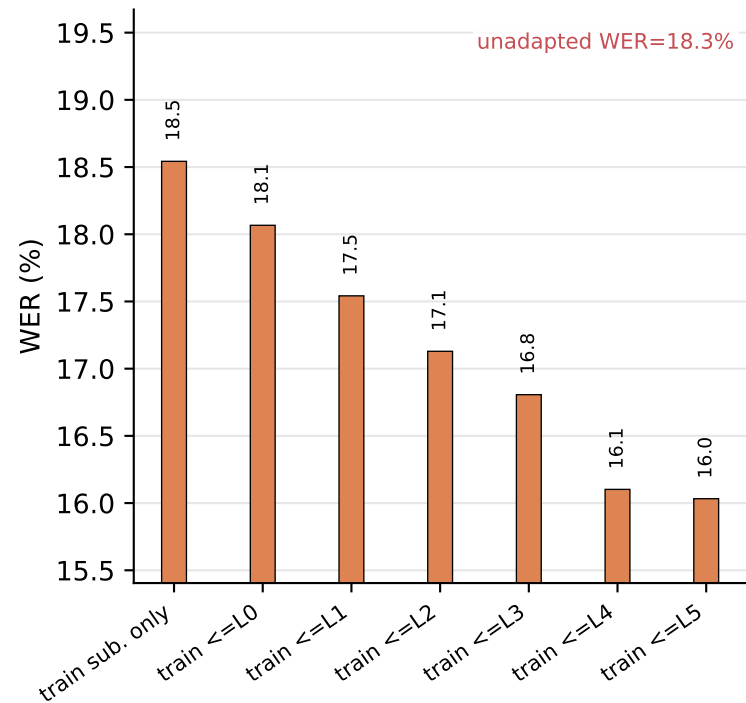
Earnings22
