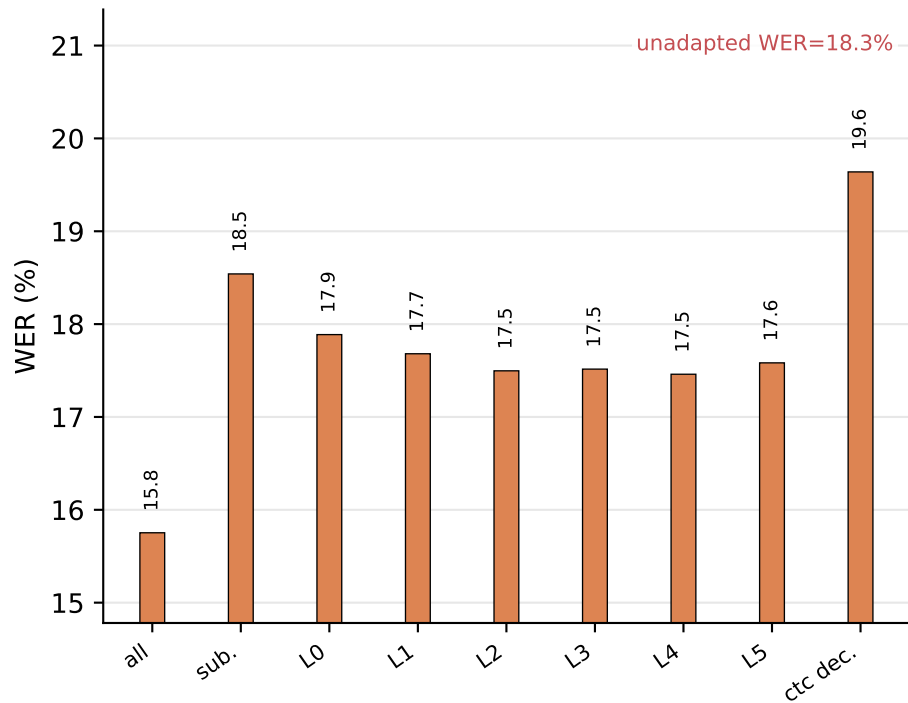
Earnings22
