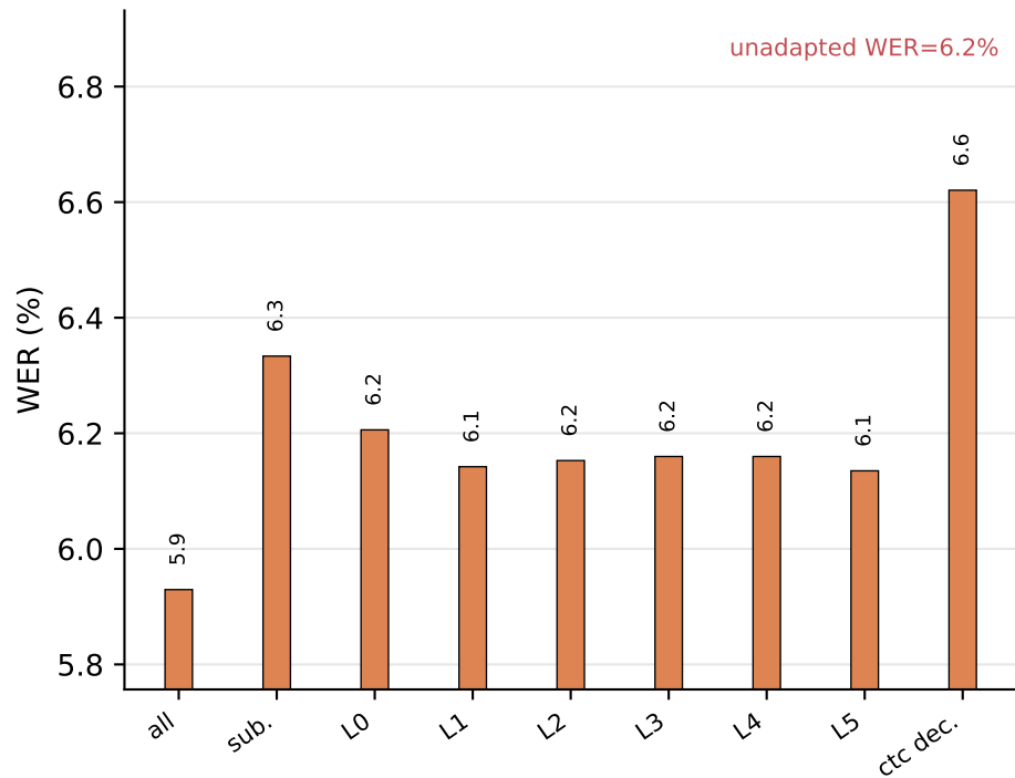
TED-LIUM
