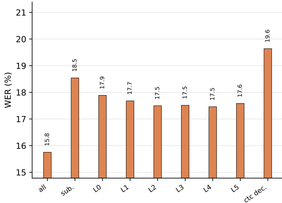
Earnings22 test
