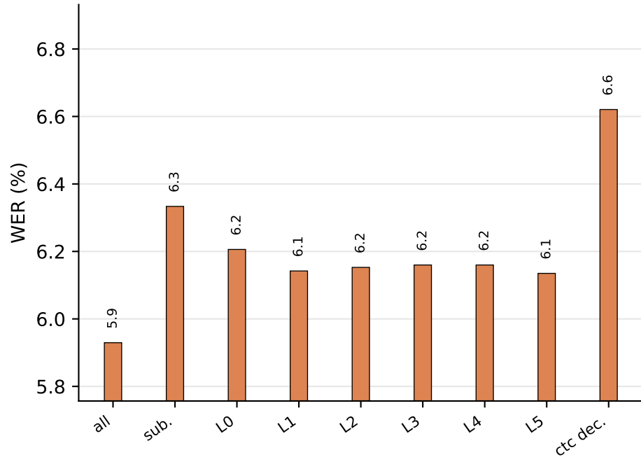
TED-LIUM test
