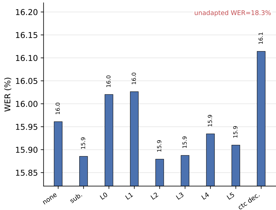
Earnings22
