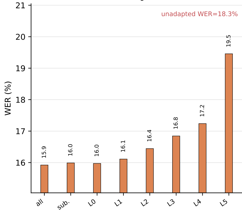
Earnings22
