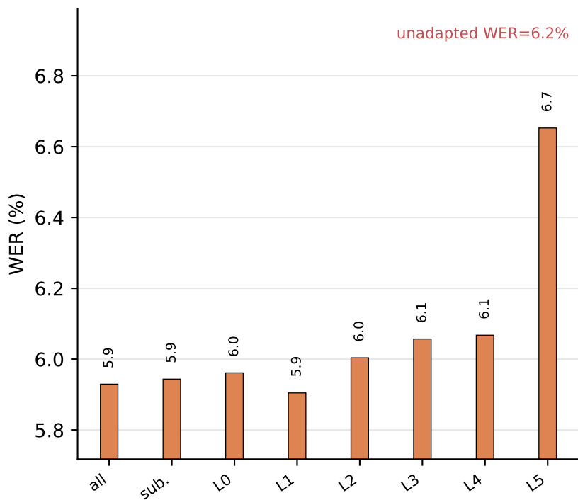
TED-LIUM
