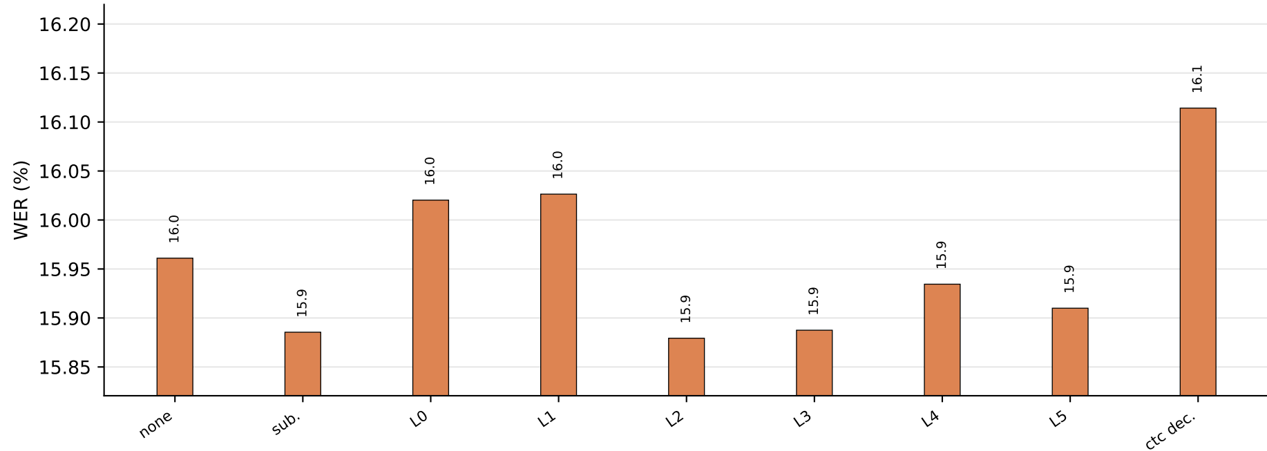
Layer-drop ablation Earnings22 test
