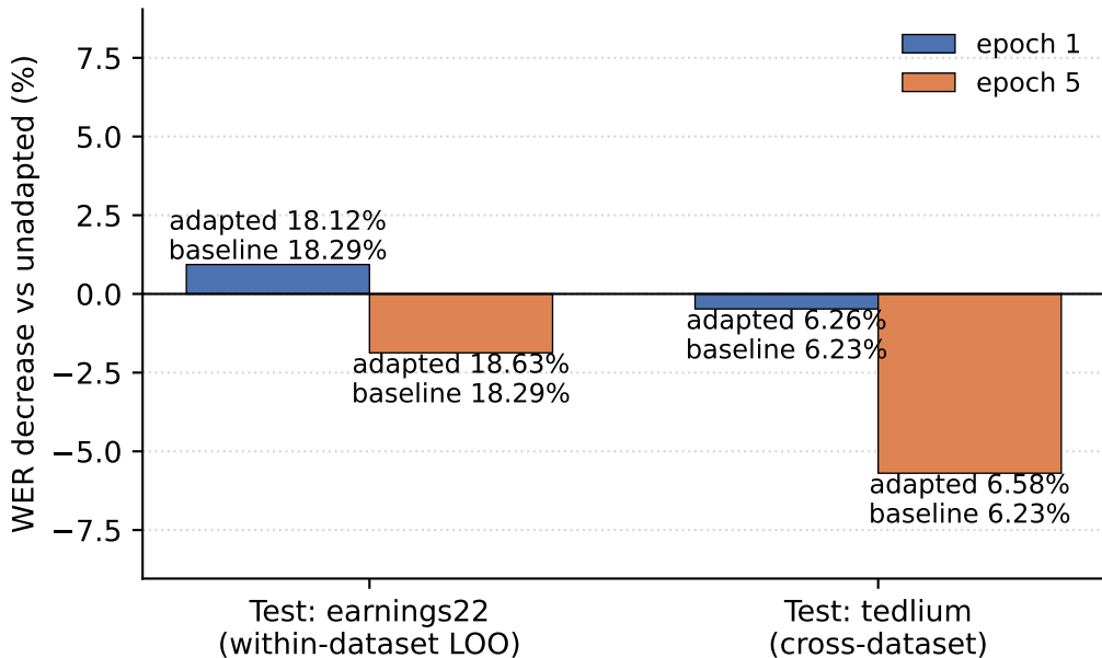
Adapt on earnings22 (epochs 1, 5, lr9e6)
