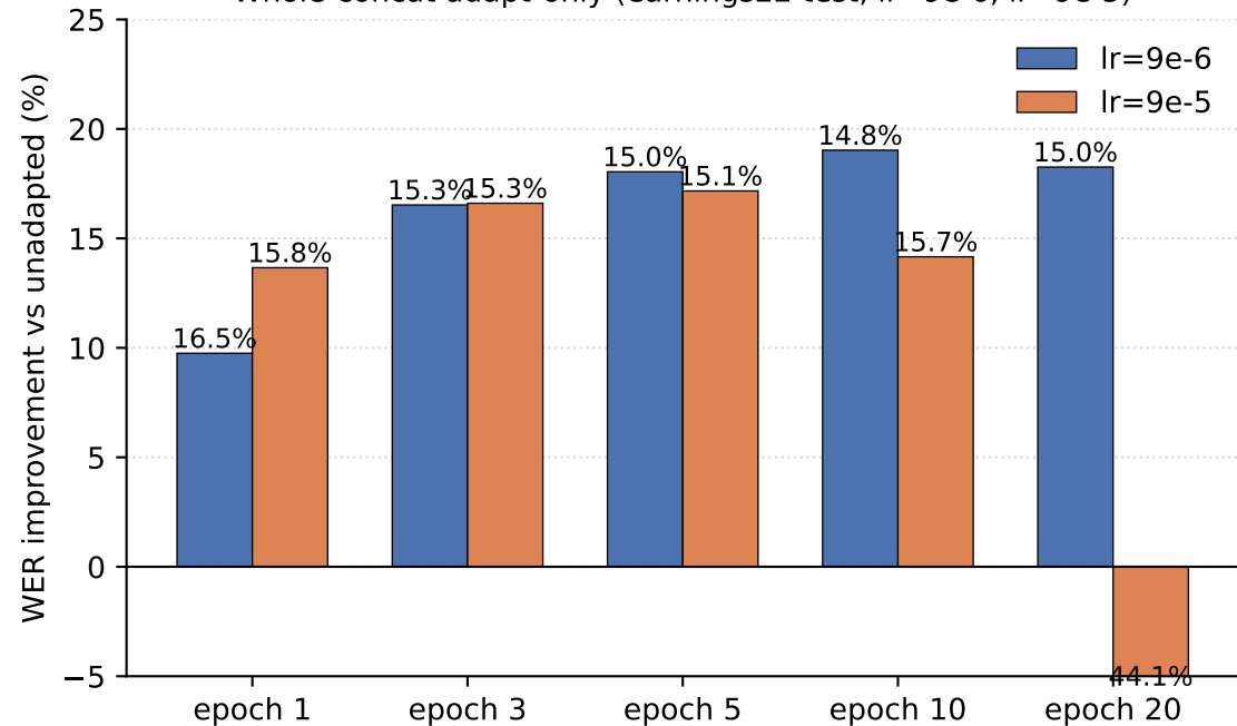
Whole-concat adapt-only (earnings22 test, lr=9e-6, lr=9e-5)
