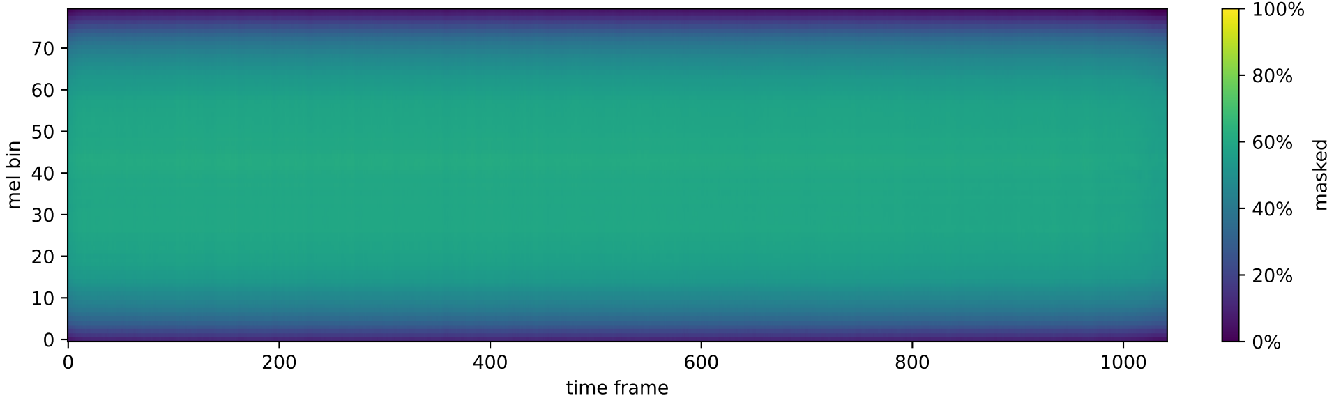
UC-MLM
