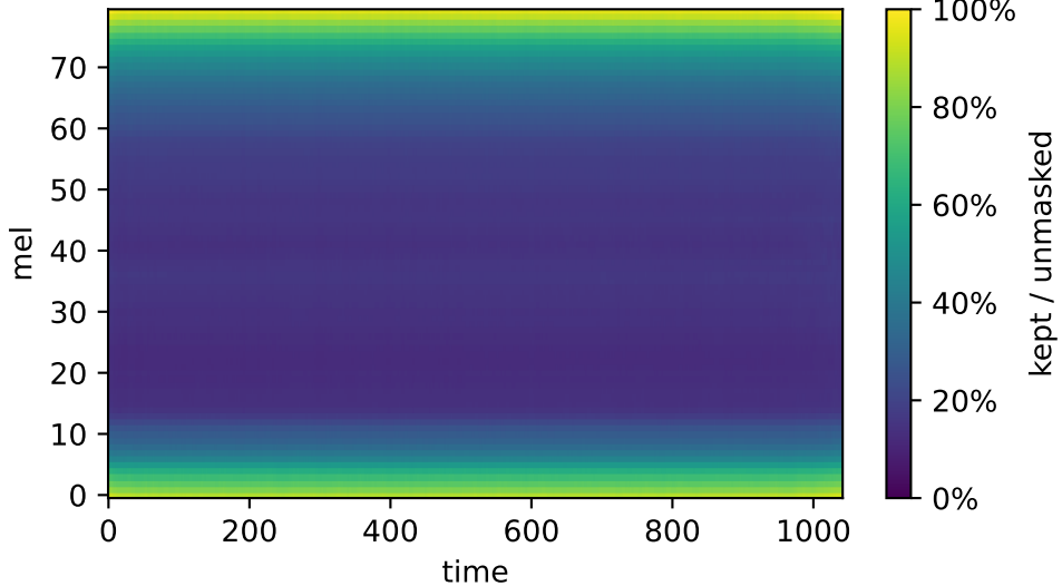
reward 0.0 keep %
