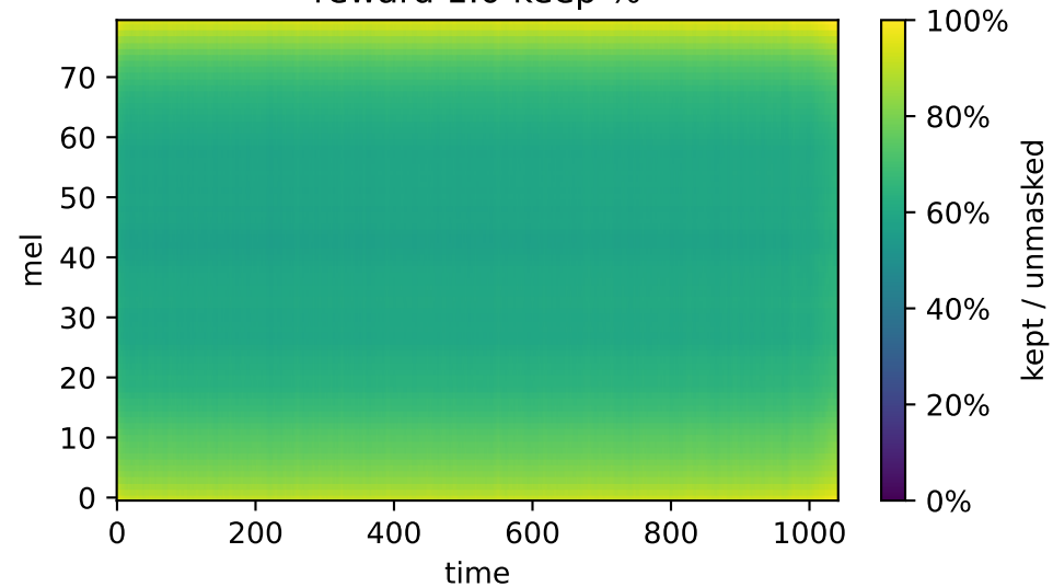
reward 1.0 keep %
