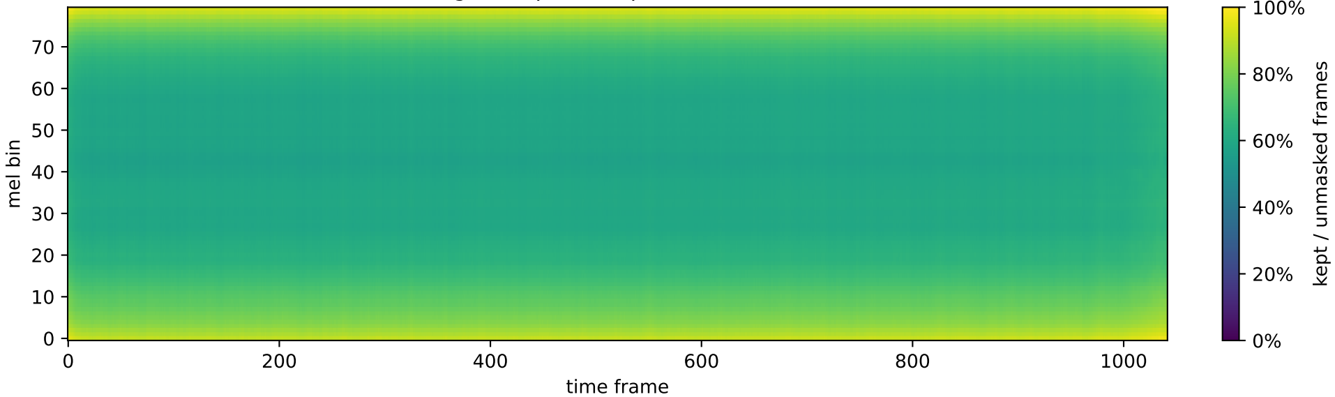
Average sampled keep mask, reward 1.0
