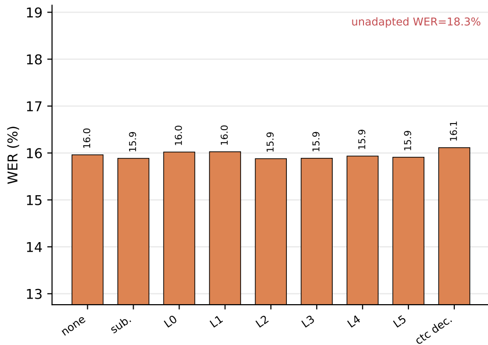
Earnings22
