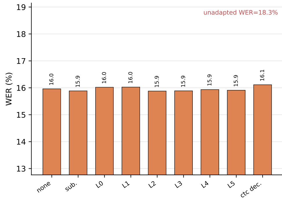
Earnings22
