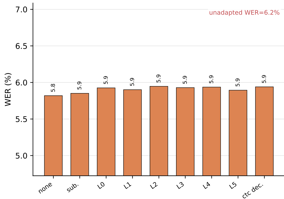
TED-LIUM
