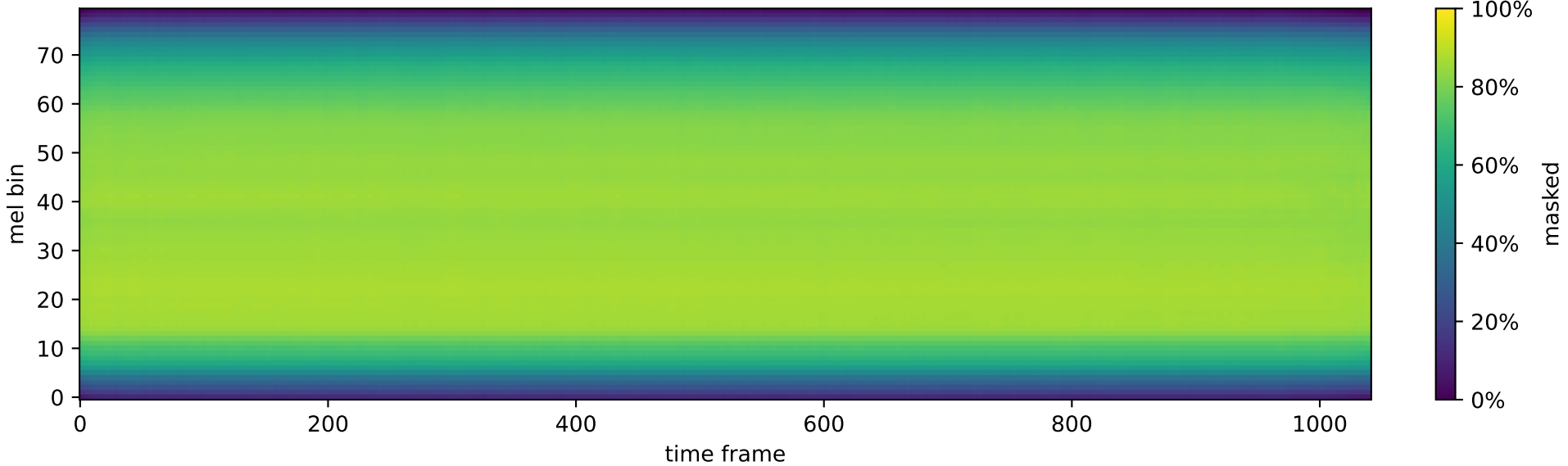
RC-MLM (reward=0.0)
