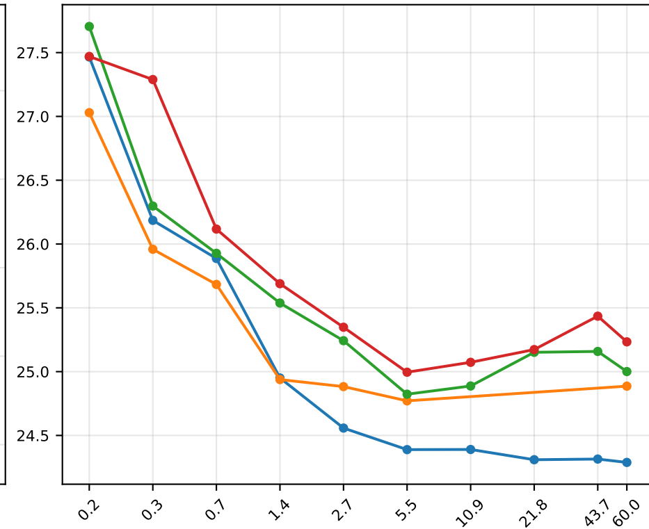
Earnings-22
