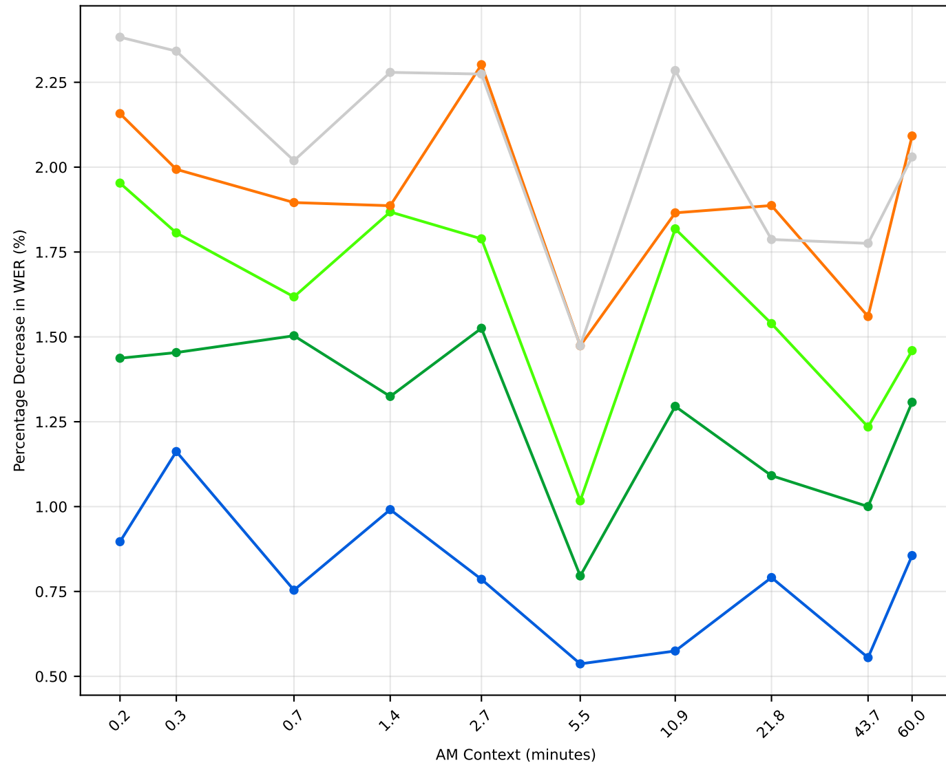
Relative Improvement over Baseline (LM=64)
