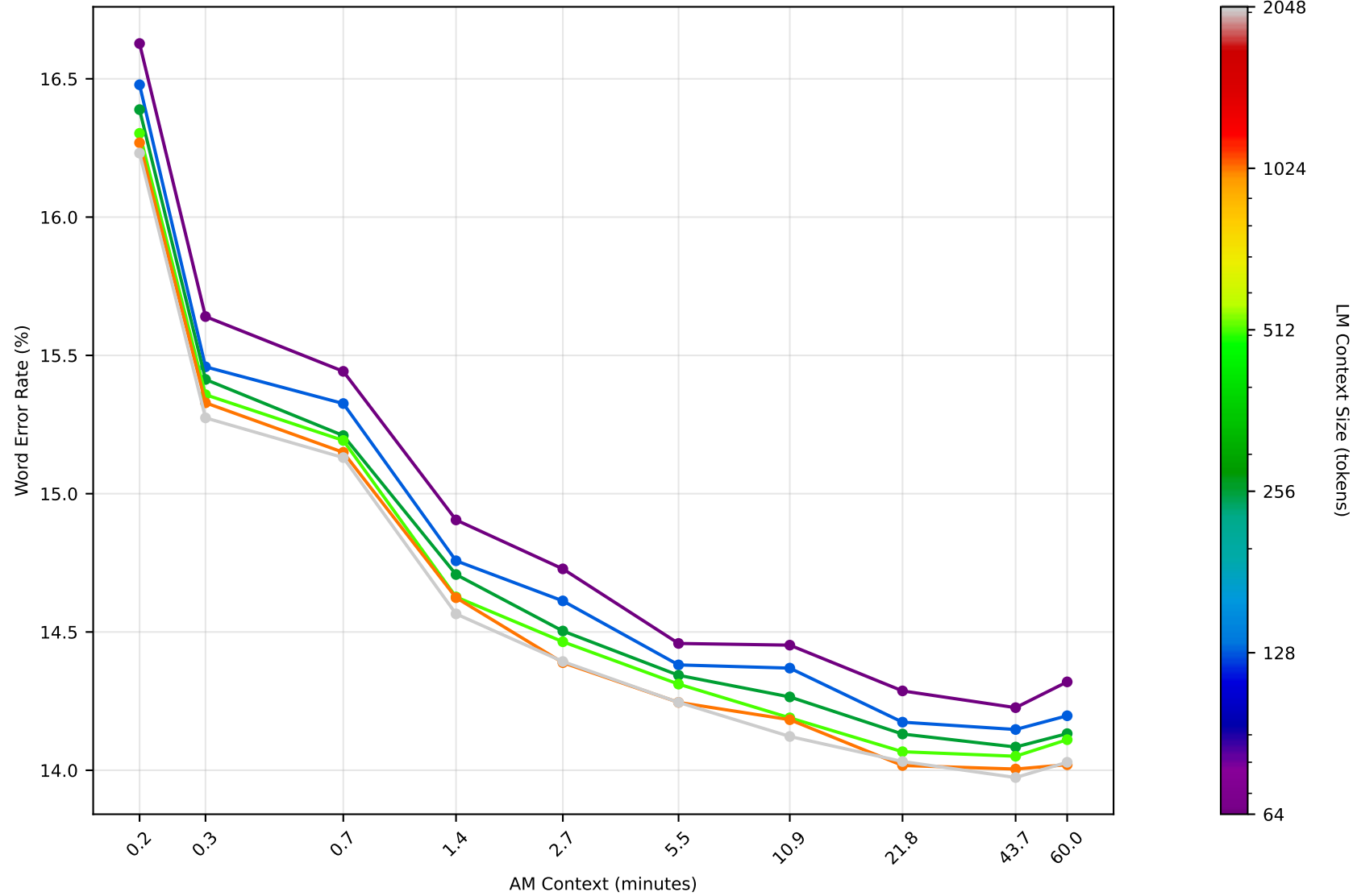
Absolute Word Error Rate
