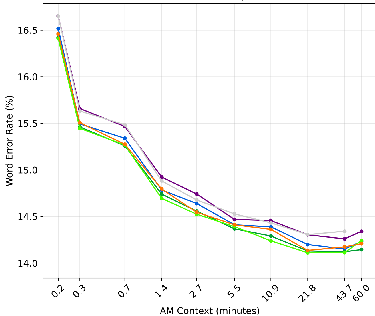
Without Prompt
