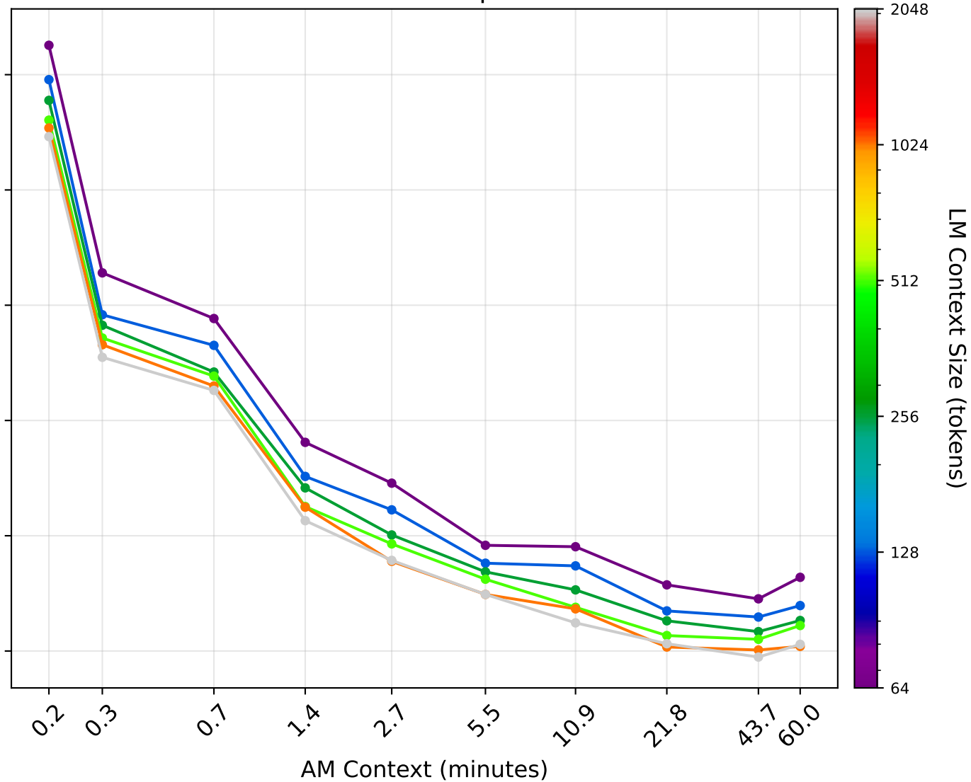
With Prompt
