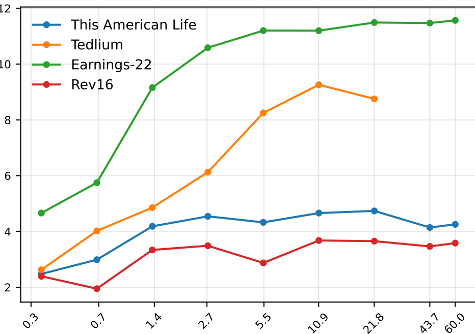
WER reduction (%) from 10s
