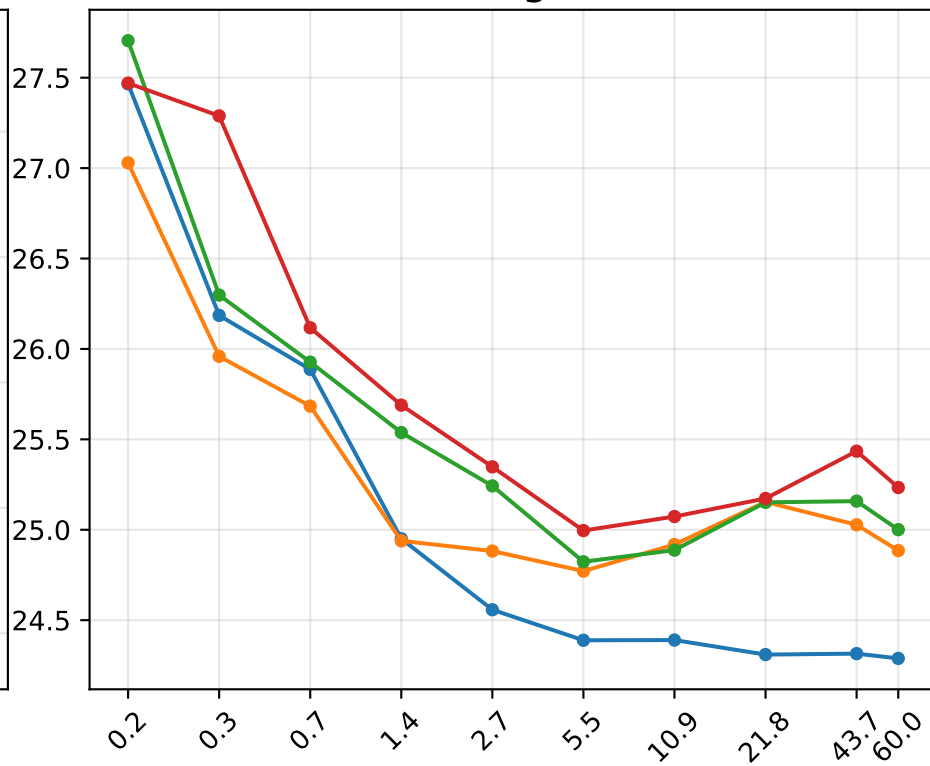
Earnings-22
