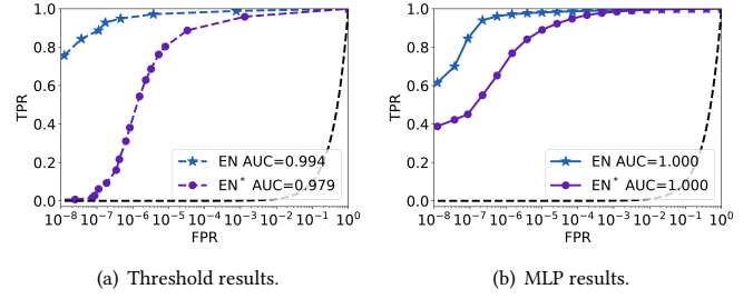
Figure 5: Comparison of the impact of CellShift-transduced and ground-truth entry-side training datasets (EN: CellShift-transduced entry-side; EN*: ground-truth entry-side. Black dashed line denotes random guessing).
