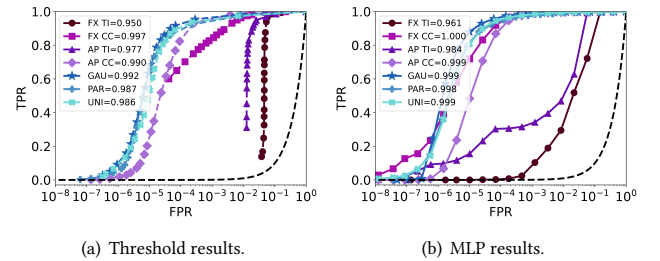
Figure 10: Performance of the ESPRESSO with various bins and kernel types (FX TI: fixed time; FX CC: fixed cell count; AP TI: adaptive time; AP CC: adaptive cell count; GAU: gaussian kernel; PAR: parabolic kernel; UNI: uniform kernel).
