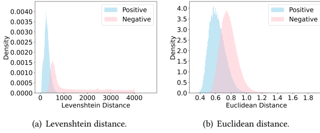
Figure 4: Comparison of the distance between t_i^{(en)} and t_i^{(en^*)} and the distance between t_i^{(en)} and t_j^{(en^*)} in a histogram.
