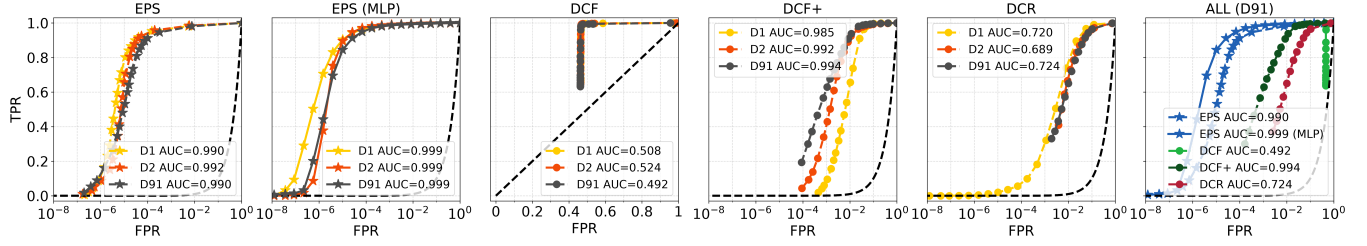
Figure 6: Thresholding performance of ESPRESSO and baselines under temporal drift. Trained with GTTCorr-Day1 and evaluated with GTTCorr-Day1 (D1), GTTCorr-Day2 (D2), and GTTCorr-Day91 (D91).
