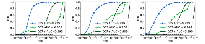
(a) Trained and evaluated with GTTCorr-All. (b) Trained with GTTCorr-All and evaluated with All-GT and CellFlow-All-GT. (c) Trained with CellFlow-All and evaluated with GTTCorr-All.
