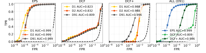
Figure 11: MLP classification performance of ESPRESSO and baselines under temporal drift. Trained with GTTCorr-Day1 and evaluated with GTTCorr-Day1, GTTCorr-Day2, and GTTCorr-Day91.
