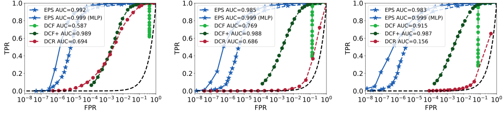
(a) Trained and evaluated with GTTCorr-All. (b) Trained with GTTCorr-All and evaluated with CellFlow-All-GT. (c) Trained with CellFlow-All-GT and evaluated with GTTCorr-All.
