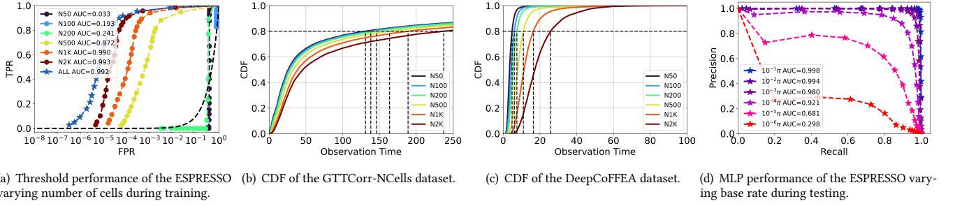
Figure 9: (a): Impact of the number of cells in the training dataset for ESPRESSO performance, (b), (c): CDF of the GTTCorr-NCells and DeepCoFFEA dataset, and (d): impact of the various base rates in the testing dataset for ESPRESSO performance.
