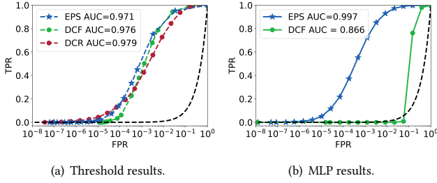
Figure 8: Performance of the ESPRESSO and baselines in the standard setting, trained and evaluated with DeepCoFFEA dataset.
