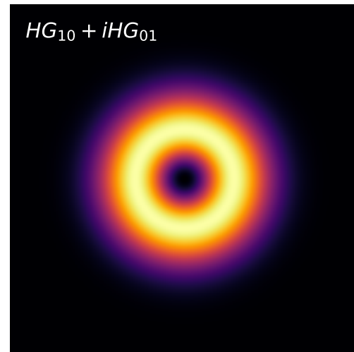
Add / subtract with \pi/2 phase
