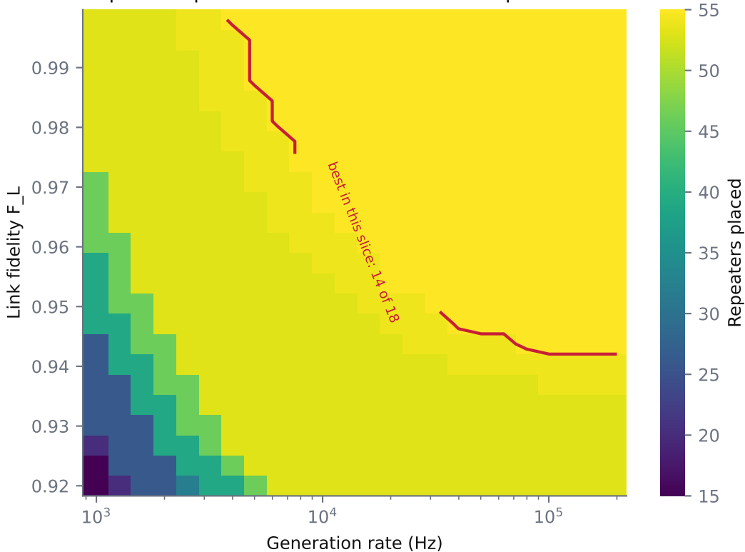
Repeaters placed over the T centre sweep box
