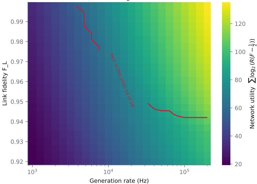
Network utility \sum \log_2 (R(F - \frac{1}{2})) over the T centre sweep box
