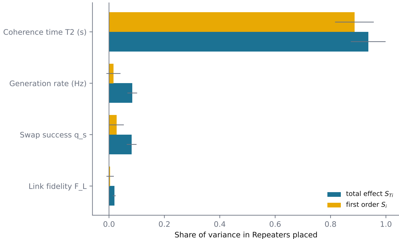
Which hardware parameter moves the result (6144 solves)
