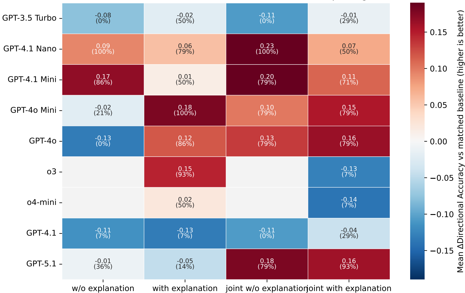
Validation Augmentation Summary: Mean \Delta Directional Accuracy Cell labels show mean delta and share of variants improving.
