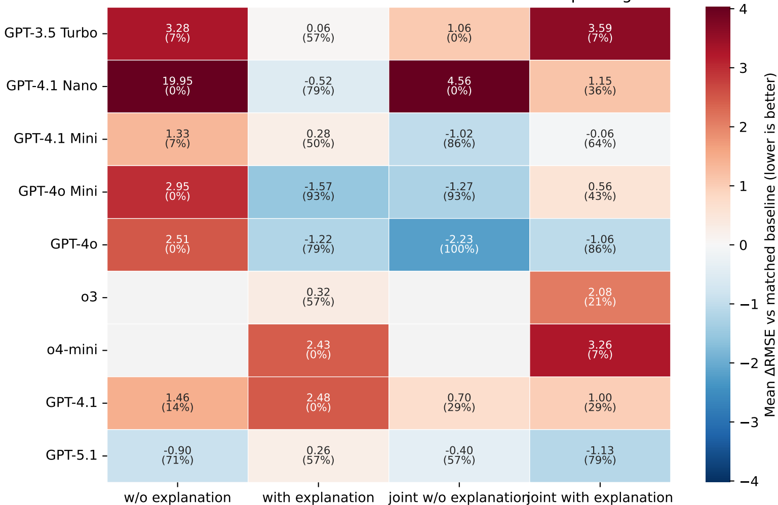
Validation Augmentation Summary: Mean \Delta RMSE Cell labels show mean delta and share of variants improving.
