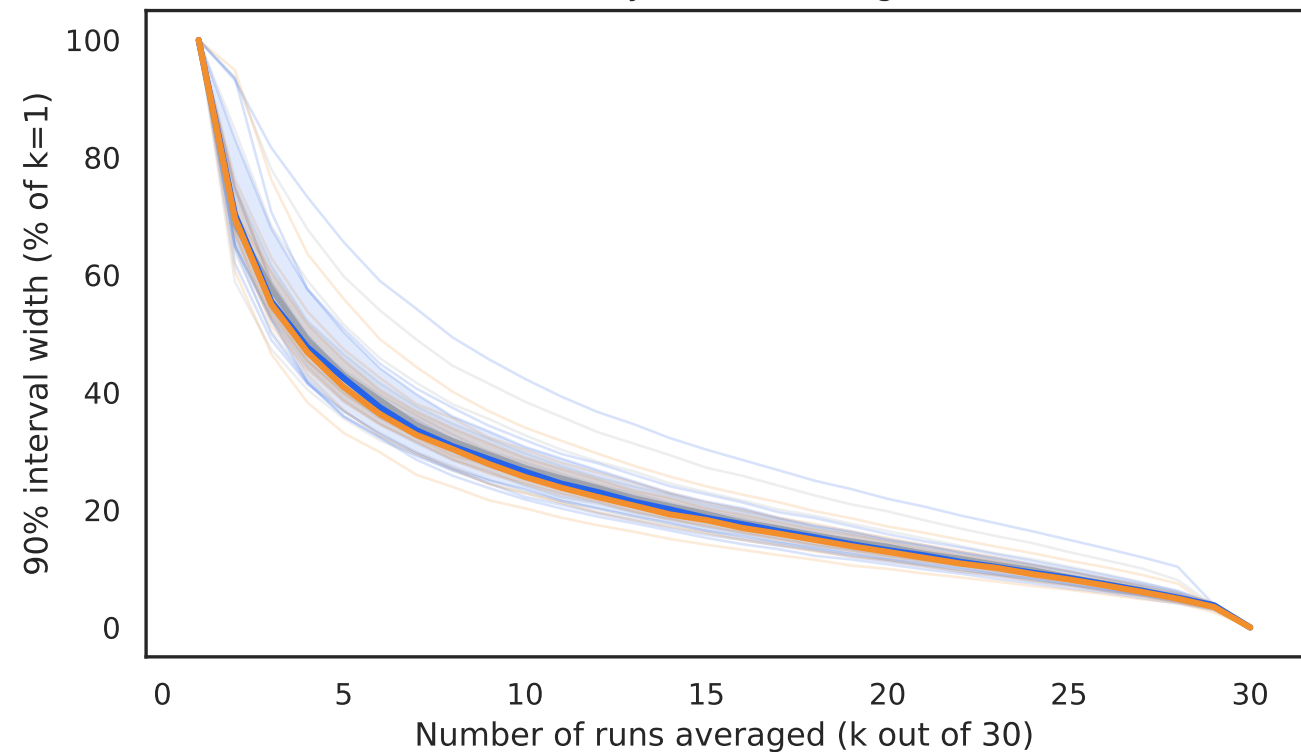
Uncertainty relative to single-run
