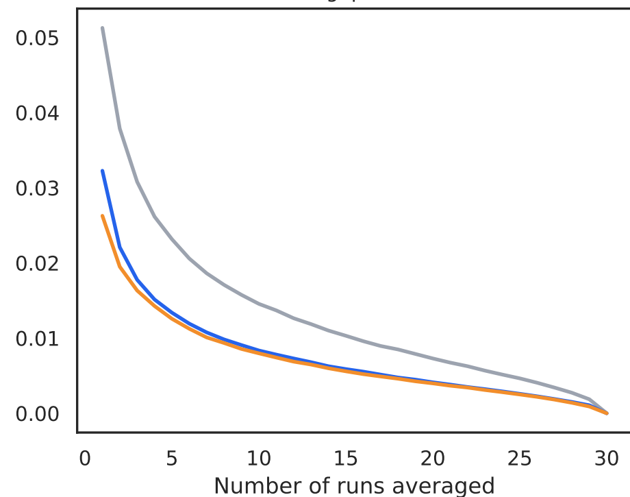
Median mean abs gap to 30-run ensemble
