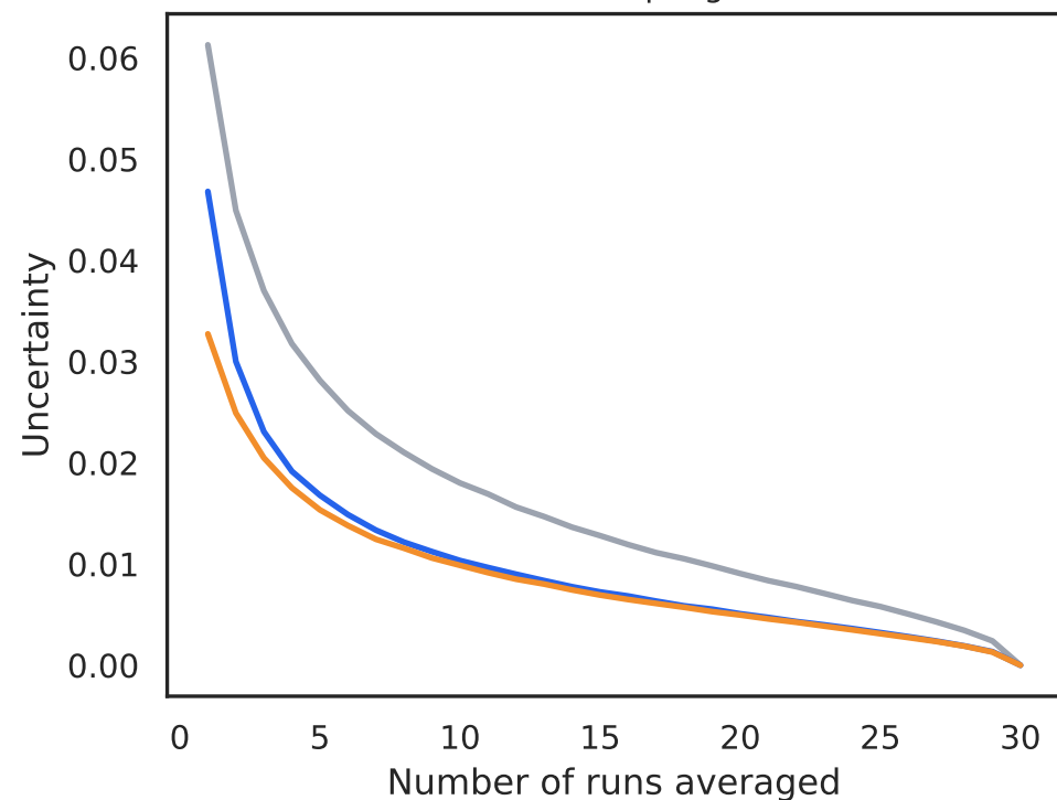
Median sampling SD
