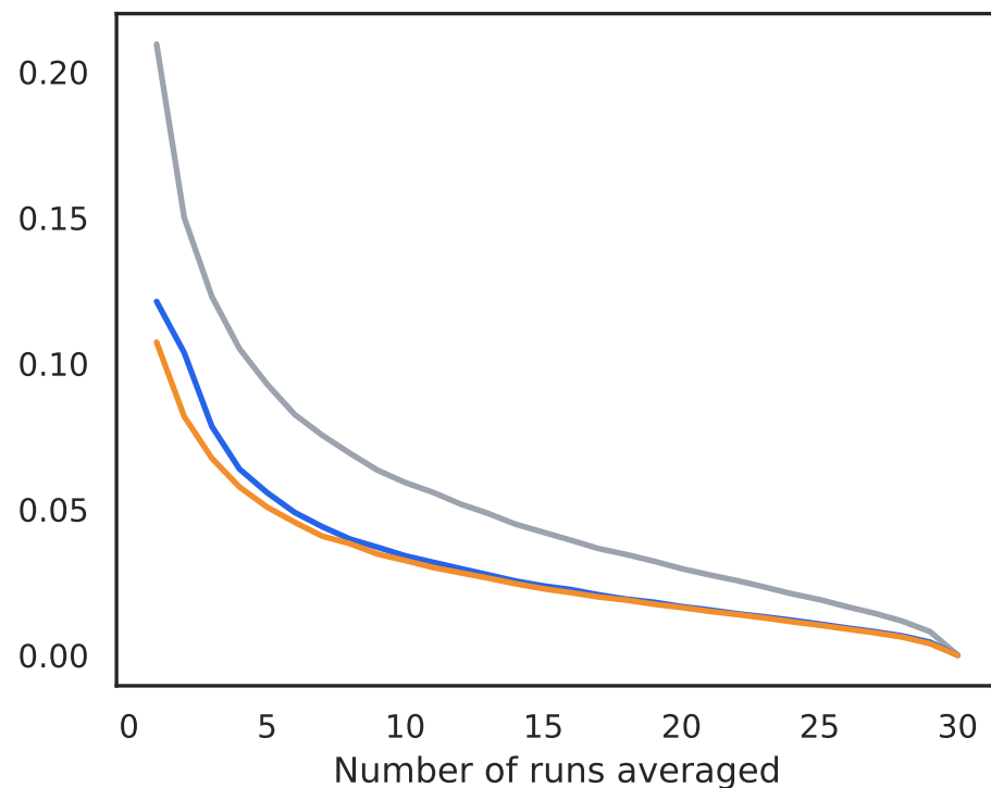
Median 90% interval width
