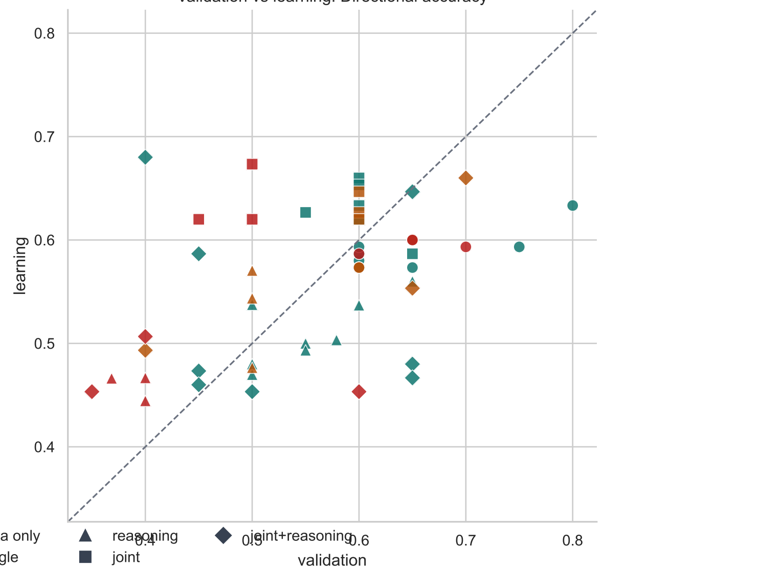
Validation vs learning: Directional accuracy
