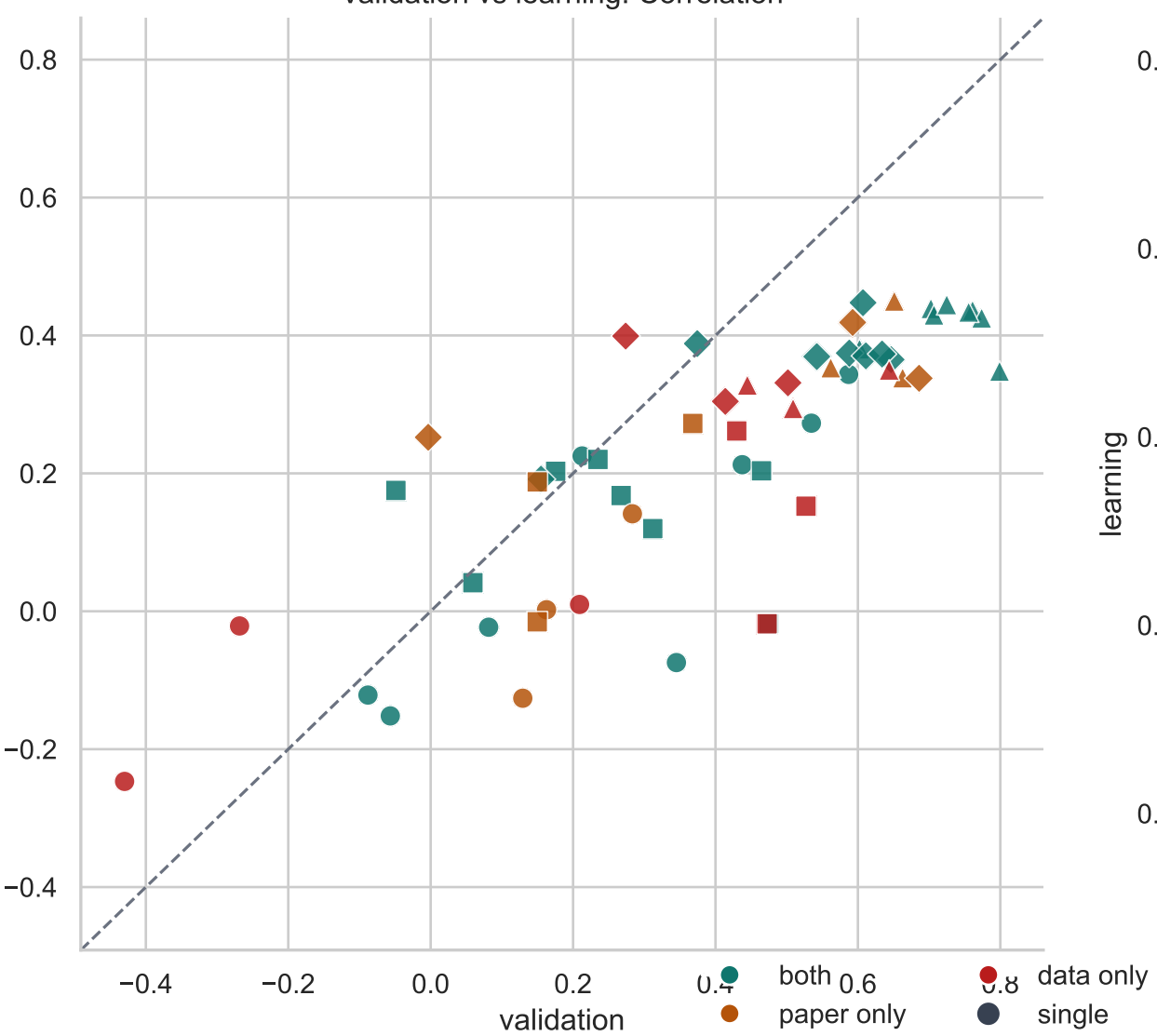
Validation vs learning: Correlation
