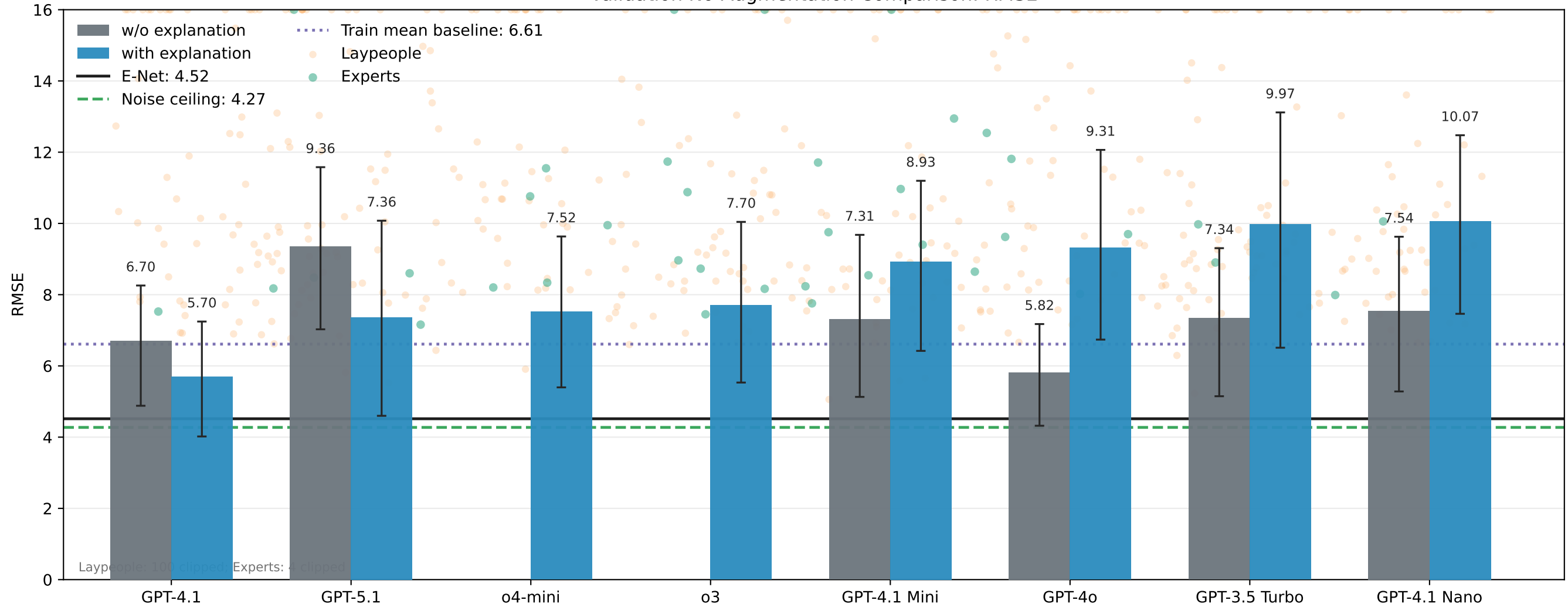
Validation No-Augmentation Comparison: RMSE
