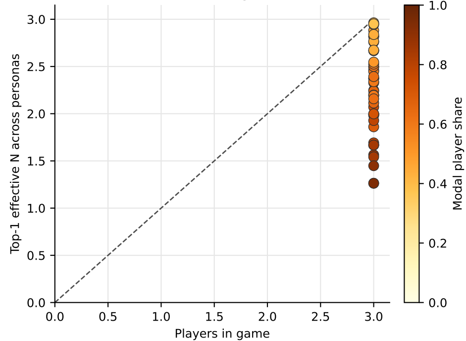
B. Effective coverage vs uniform
