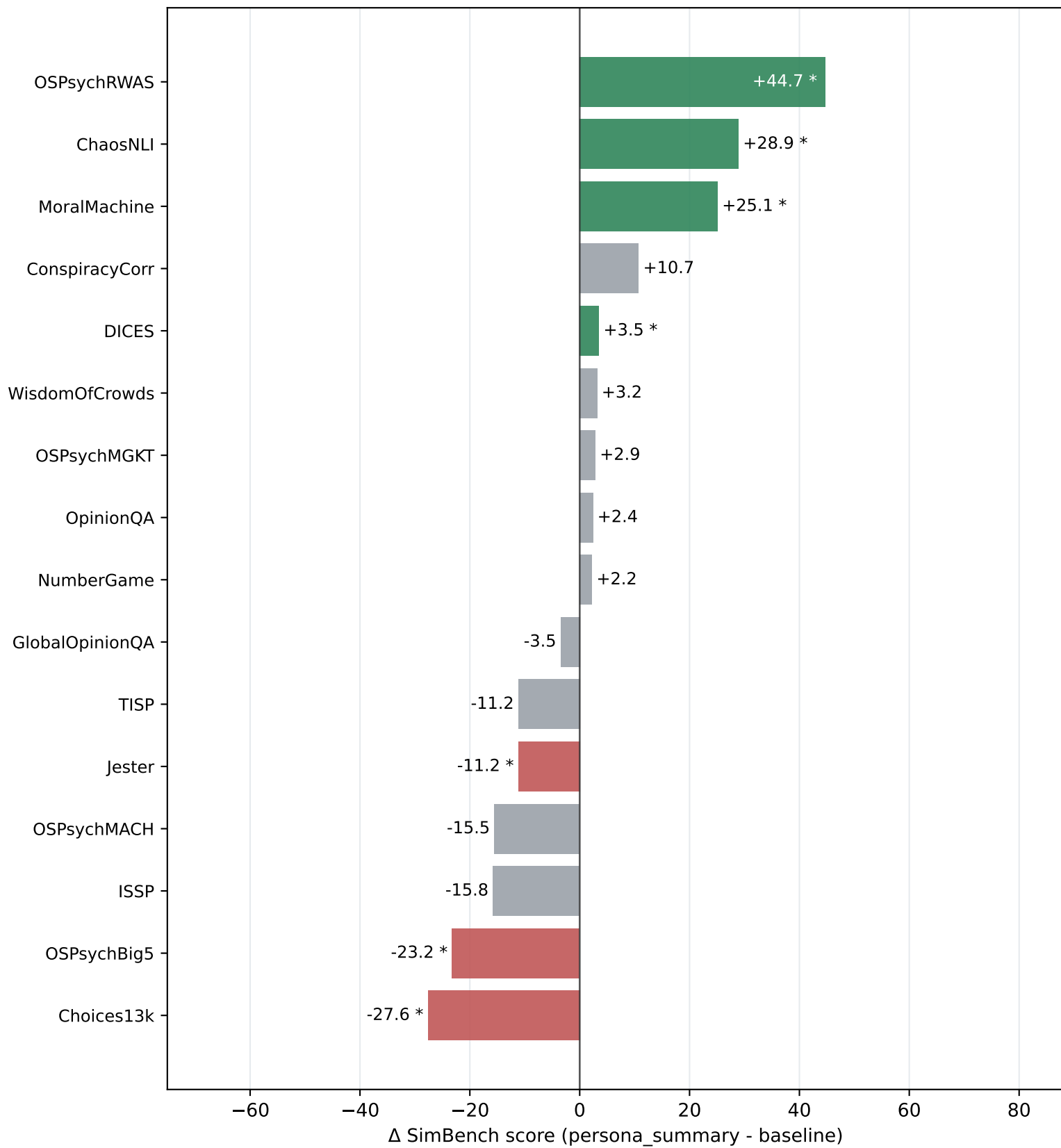
gpt-5-mini
