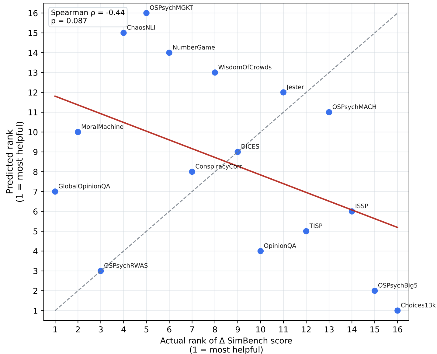
gpt-5-mini
