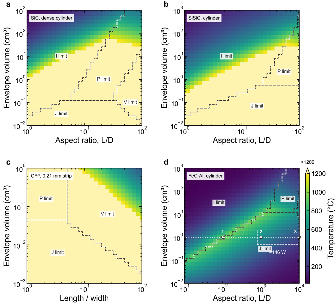
Figure S5. Lumped material screening under 150 V, 40 A and 2 kW limits: (a) dense SiC cylinder, (b) SiSiC cylinder, (c) CFP strip of 0.21 mm thickness and (d) FeCrAl cylinder.
