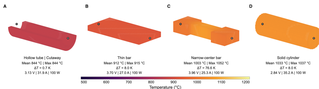
Figure 5. Steady temperature fields for four SiSiC geometries at 100 W: (A) hollow tube, (B) thin bar, (C) narrow-center bar, (D) solid cylinder. Panels are ordered by volume-average temperature and share the same viewing angle and 500–1200 °C color scale. The hollow tube uses a longitudinal half-cutaway; all reported temperatures refer to the complete body. \Delta T is the maximum minus minimum solid temperature. Solid volumes are 1.000–1.021 \text{cm}^3 . Images are captured from the browser-calculated fields.
