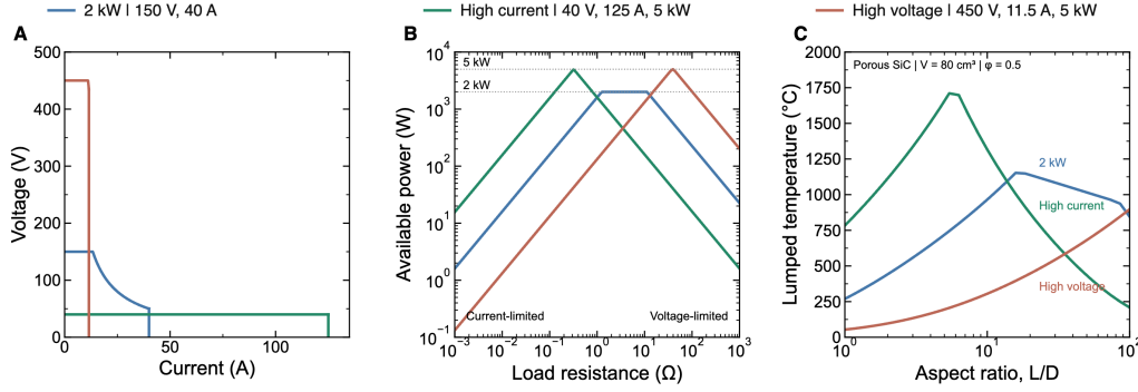
Figure S6. Power-supply selection from electrical ratings to predicted temperature. (A) Positive-quadrant upper operating boundaries for the 62020H-150S (blue), 62050H-40 (green) and 62050H-450 (red), using nominal voltage, current and power ceilings. (B) Available power versus load resistance, \min(I_{\max}^2 R, V_{\max}^2 / R, P_{\max}) , before material current-density limits. Low resistance is current-limited and high resistance is voltage-limited. (C) Lumped temperatures for porous SiC at an 80 \text{ cm}^3 envelope volume and 0.5 solid fraction as L/D varies; preset current-density limits are included. Colors identify the same supplies in all panels. The compared supplies have different rated powers. Dynamic response, ripple and derating are not modeled.
