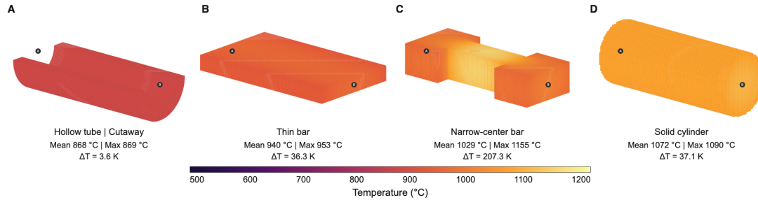
Figure S8. Steady temperature fields for four FeCrAl geometries at 100 W: (A) hollow tube, (B) thin rectangular bar, (C) bar with a narrow center, and (D) solid cylinder. Panels are ordered by volume-average temperature and share the same viewing angle and 500–1200 °C color scale. Panel A uses a longitudinal half-cutaway; all reported temperatures refer to the complete body. \Delta T is the maximum minus minimum solid temperature.
