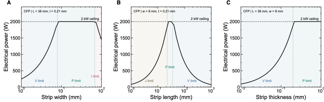
Figure S4. Electrical constraints during dimensional sweeps under 150 V, 40 A and 2 kW supply ceilings and the preset current-density limit. Shaded regions identify the active constraint at each calculated operating point; dotted boundaries are placed between adjacent samples. I, J, P and V denote current, current-density, power and voltage limits, respectively. (A) CFP width at fixed length and thickness. Increasing width lowers resistance, shifting operation from voltage limitation through the power ceiling to current limitation. (B) CFP length at fixed cross-section. Power increases under the current-density limit, reaches the power ceiling and decreases under the voltage limit. (C) CFP thickness at fixed length and width. Increasing thickness reduces resistance until the power ceiling is reached. All panels report electrical power. Dimensional changes also affect mass and exposed area, so temperature requires a thermal calculation. The electrical comparisons include cases above 1200 °C.
