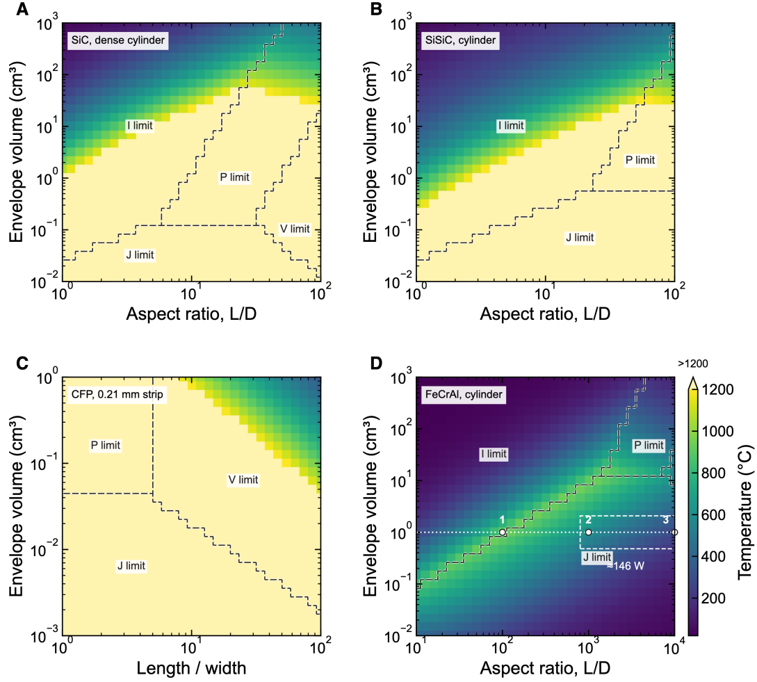
Figure S5. Lumped material screening under 150 V, 40 A and 2 kW limits. (A) Dense SiC cylinder. (B) SiSiC cylinder. (C) CFP strip of 0.21 mm thickness. (D) FeCrAl cylinder. Pale yellow indicates temperatures above 1200 °C. Dashed boundaries separate the active electrical constraints: I, current; J, current density; P, power; V, voltage. The CFP panel uses length-to-width ratio and a separate volume range.
