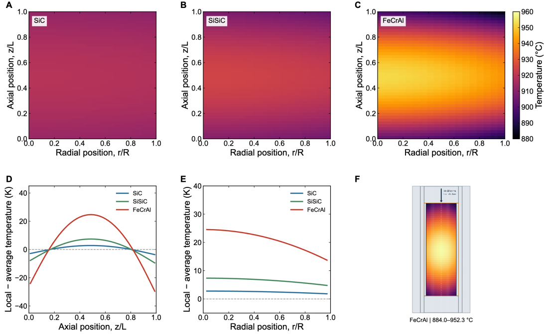
Figure 3. Material-dependent temperature distributions at a 900 °C lumped temperature. Dense cylinders have volume 1.18 \text{ cm}^3 , L/D = 3 , length 23.82 mm and diameter 7.94 mm. Each material uses its own current setpoint. (A–C) SiC, SiSiC and FeCrAl solid temperature fields on the same color scale. The radial and axial coordinates are independently normalized. (D) Centerline axial and (E) midplane radial temperatures relative to the respective volume averages. Lines connect calculated cell-center values. (F) ScreenJoule 2D thermal map calculated with the same FeCrAl inputs; the full reactor domain retains physical proportions and the application’s element-focused color mapping. The calculated mean and maximum are 927.6 and 952.3 °C. Panels A–E use the study fields archived with the calculation data. Resistivity and emissivity also differ among presets; conductivity is constant for SiC and FeCrAl and tabulated for SiSiC. Table S2 records input assumptions and operating points.
