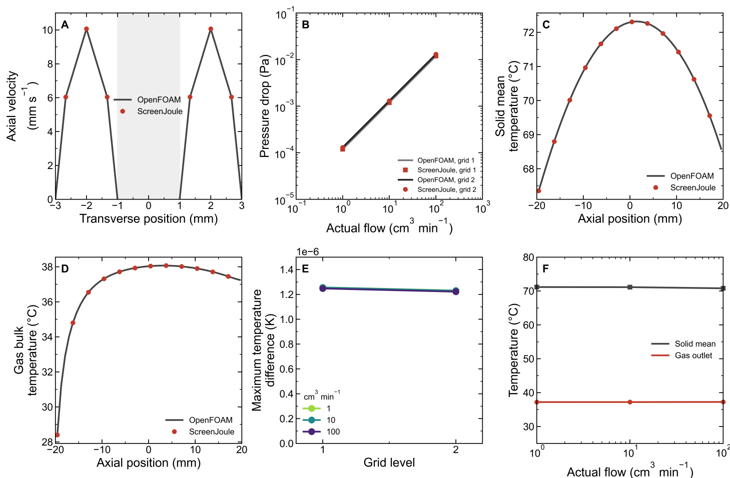
Figure S9. OpenFOAM comparison of fully developed flow and conjugate heat transfer. (A) Axial velocity across the channel height, averaged over the two gas columns nearest the width centre; shading marks the solid and lines include the no-slip boundary values. (B) Pressure drop versus actual flow rate on both meshes. (C,D) Solid section-mean and flow-weighted gas temperatures along the channel. Panels A, C and D use 100 cm 3 min -1 on the finer mesh. (E) Maximum cell-temperature difference between codes at each grid level. (F) Solid mean and gas outlet temperatures on the finer mesh. Lines denote OpenFOAM and symbols denote ScreenJoule in A–D and F. Grid levels 1 and 2 are 12 × 9 × 24 and 24 × 9 × 48.
