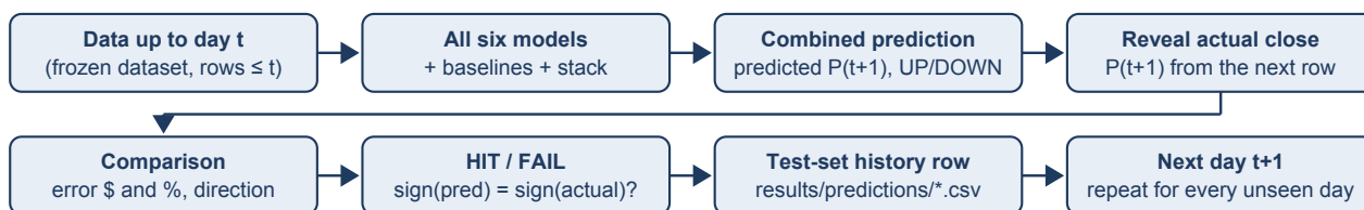
Figure 10. The verification loop implemented for the unseen test period (src/evaluation/backtesting.py :: main; interactively: prediction.py :: predict_for_date).
