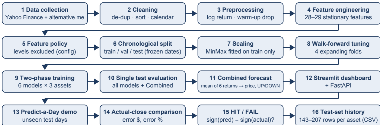
Figure 1. The implemented pipeline. Stages 1–7 live in src/data/ , 8–9 in src/training/ , 10 and 16 in src/evaluation/backtesting.py , 11 and 13–15 in src/inference/prediction.py , 12 in app/streamlit_app.py and src/api/app.py .
