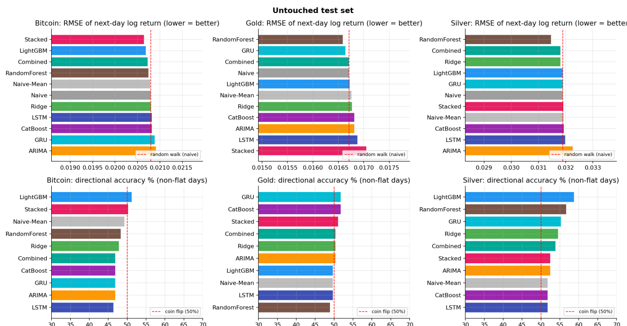
Figure 7. Test-set RMSE of the next-day return and directional accuracy for every model and asset (results/figures/model_comparison_test.png). The RMSE axes are zoomed: all models lie within \pm 1\% of the random walk.
