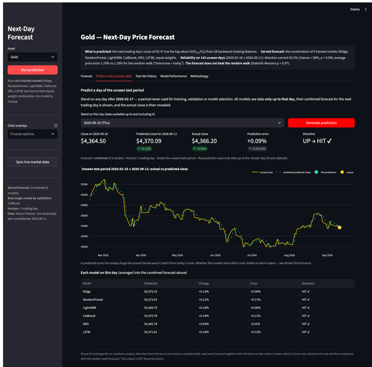
Figure 12. Predict a Day (unseen test): the combined forecast for the day after 2026-09-10 made from data up to that day, the revealed actual close, error and HIT, and each member on that day.
