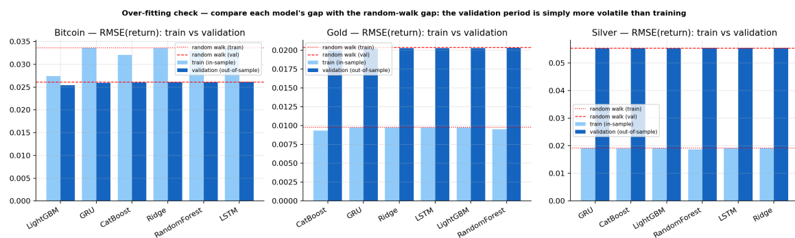
Figure 6. Train vs validation RMSE per model and asset (results/figures/overfitting_gap.png).
