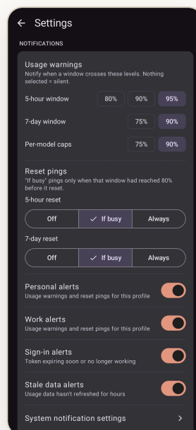
Granular alert controls – chips & reset-ping modes
