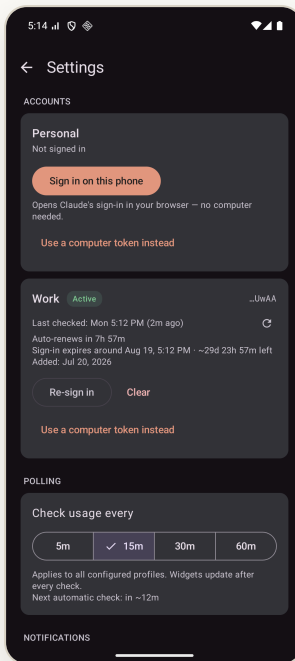
1 – Each account card has "Sign in on this phone"
