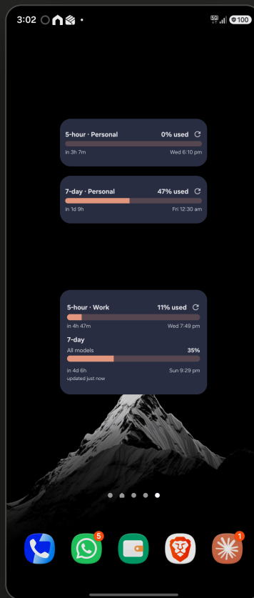
Home-screen widget
