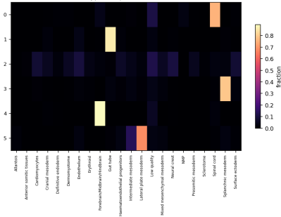
Niche x cell-type composition (row-normalised)
