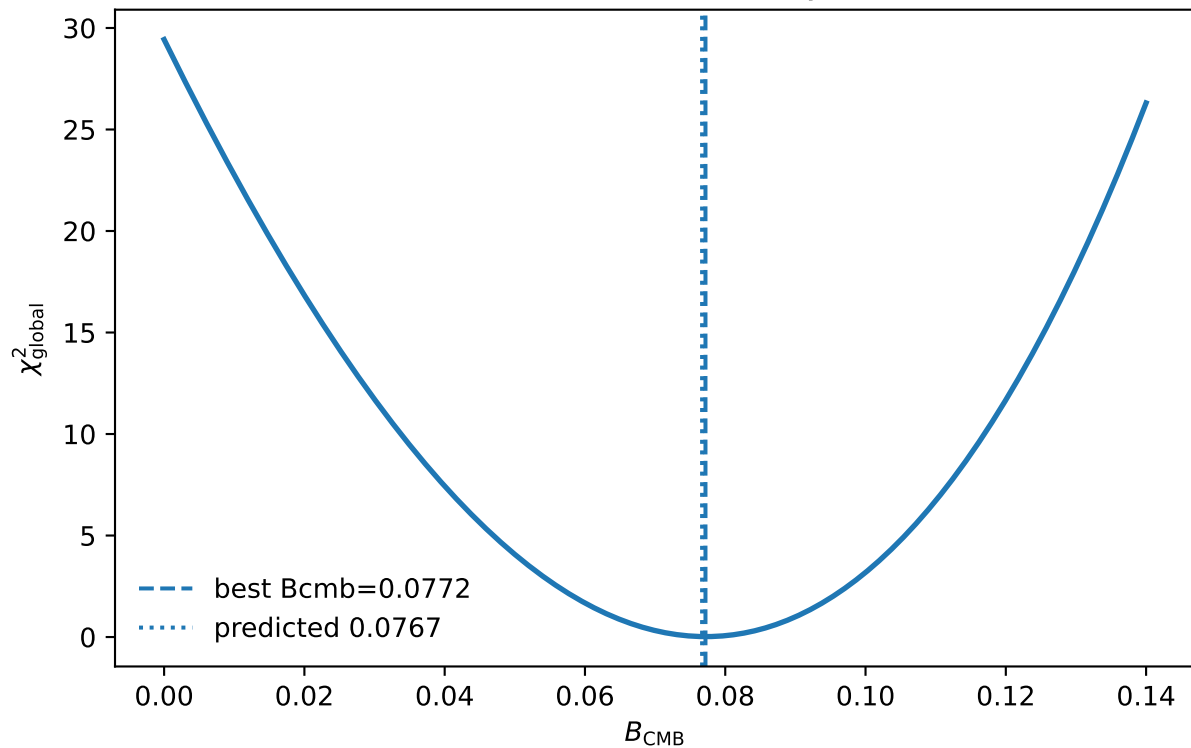
Global Hubble consistency scan
